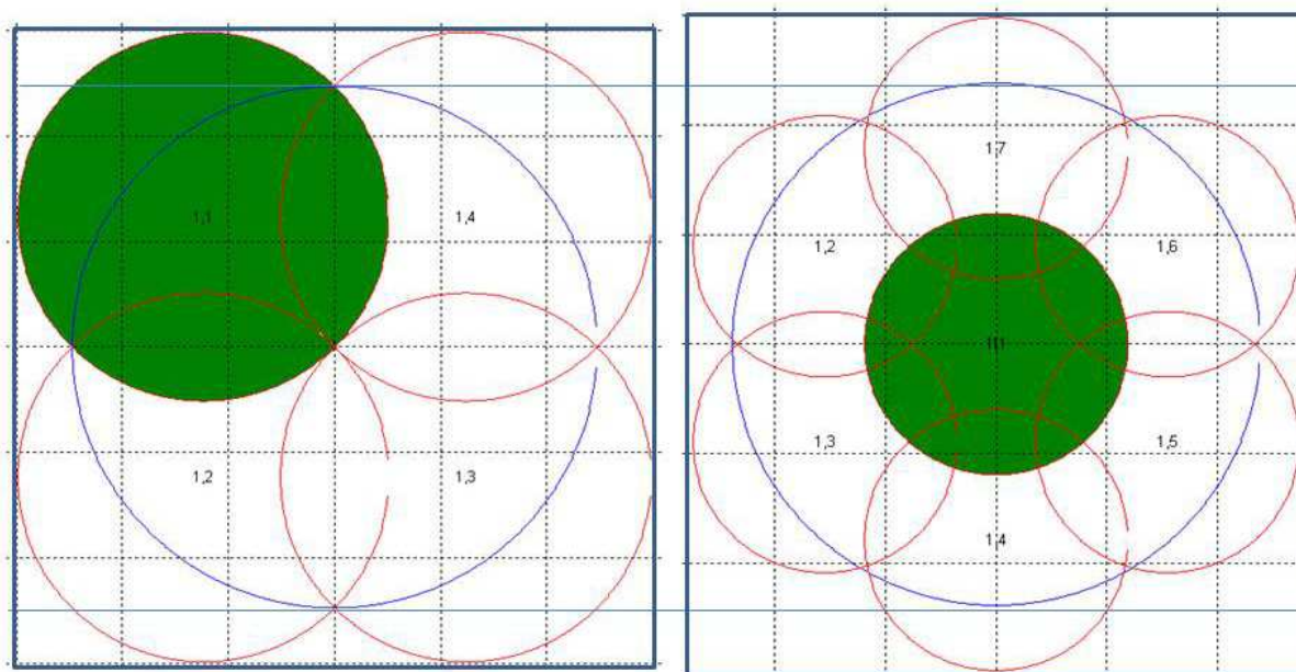
Fig. 24. Sub-beam selection for interference calculations, N_s = 4
