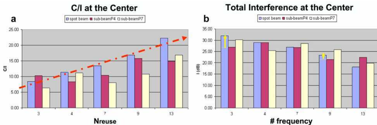
Fig. 25. Interference at the center by tier for sub-bem partition=4, 7 and frequency reuse 3, 4, 7, 9, 13. (a) C/I (b) Total interference
