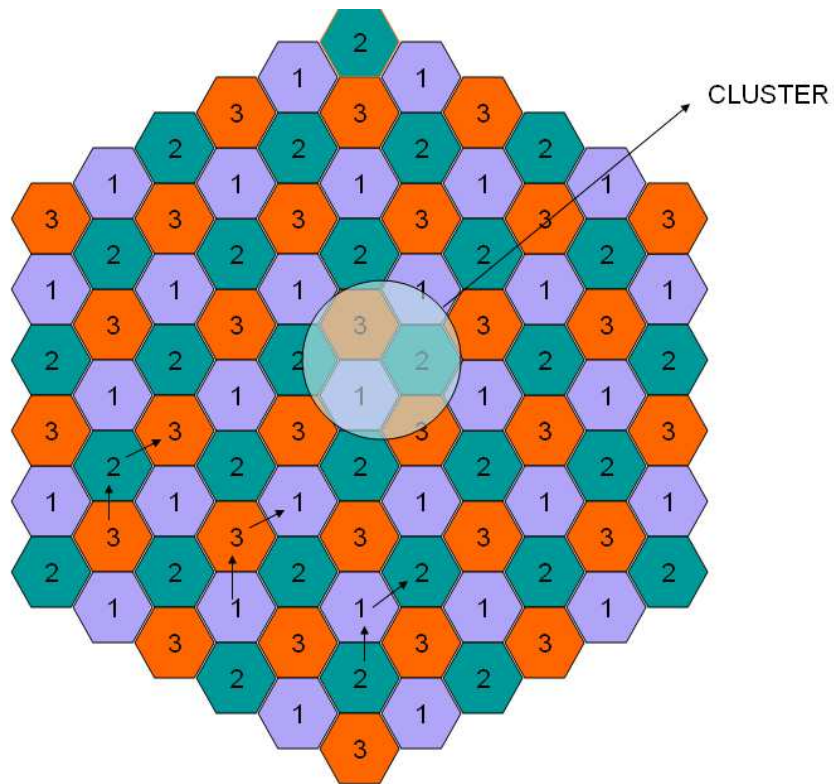
Fig. 6. Cluster coverage, N=3
