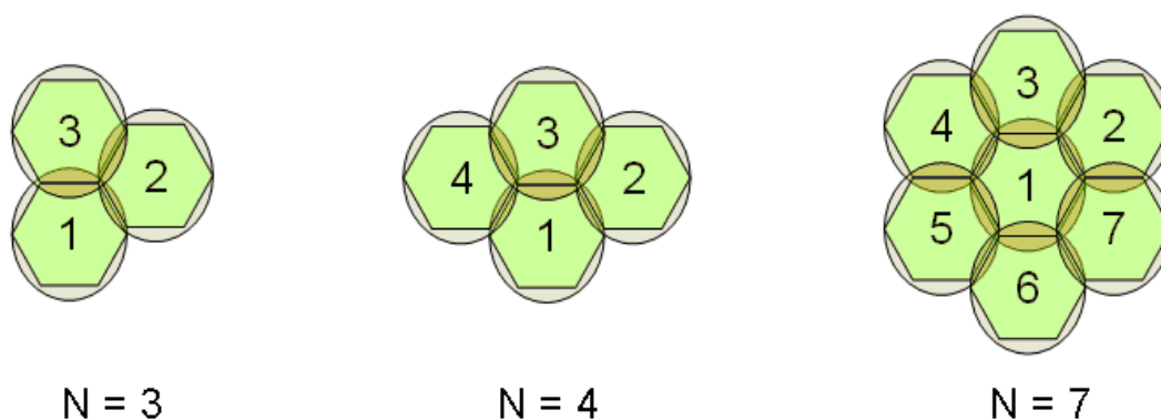
Fig. 5. Different cluster options for hexagonal lattice
