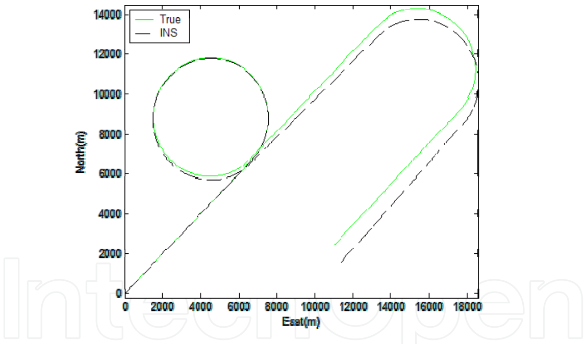
Fig. 11. Trajectory for the simulated vehicle (solid) and the INS derived position (dashed)
