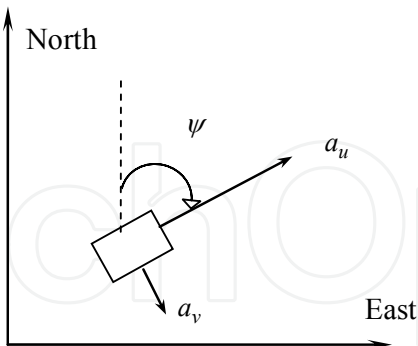
Fig. 3. Two-dimensional inertial navigation, Farrell & Barth (1999)
