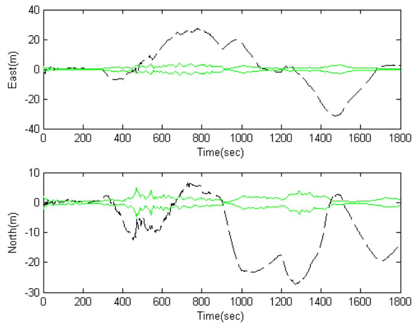
Fig. 17. East and north components of navigation errors and the 1-σ bound based on the proposed method when the threshold setting is not incorporated
