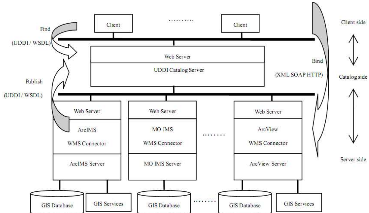
Fig. 7. the Geo-information Sharing Architecture Based on WMS
