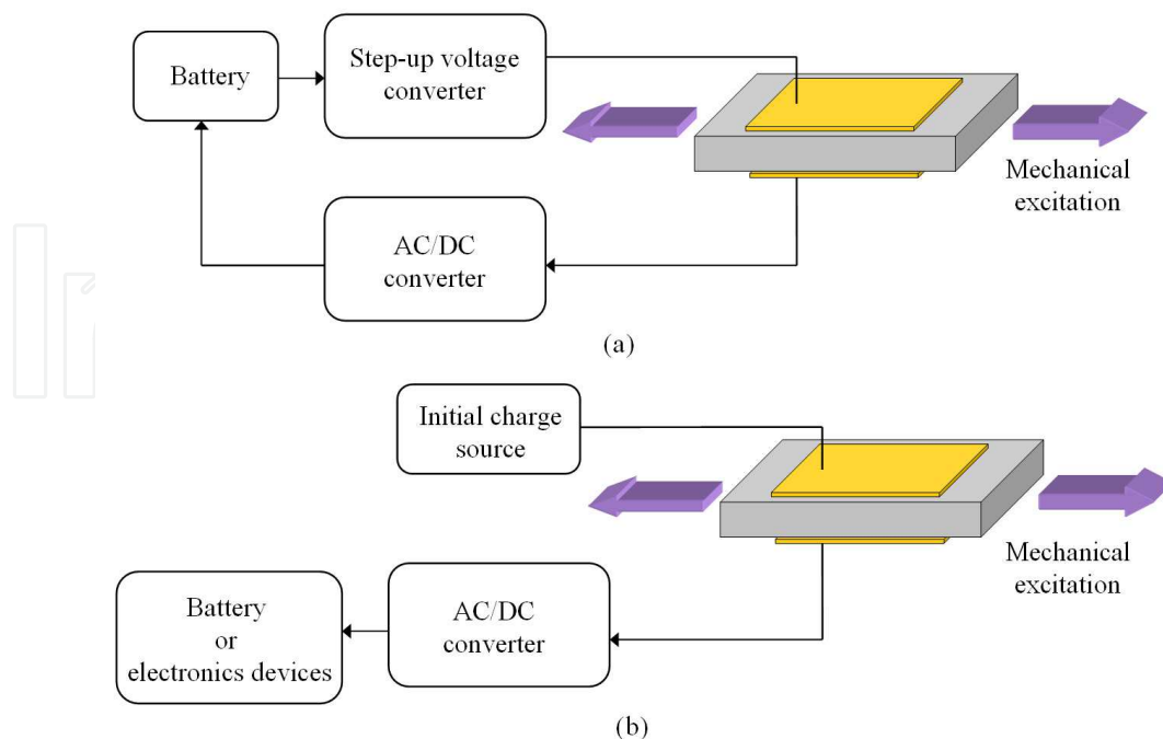
Fig. 12. Two conceptual circuit topologies for electrostrictive polymers generators
