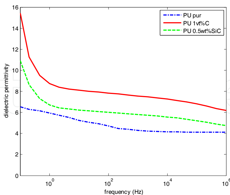
Fig. 7. The variation in the dielectric constant for a pure PU material and filled composite vs frequency.
