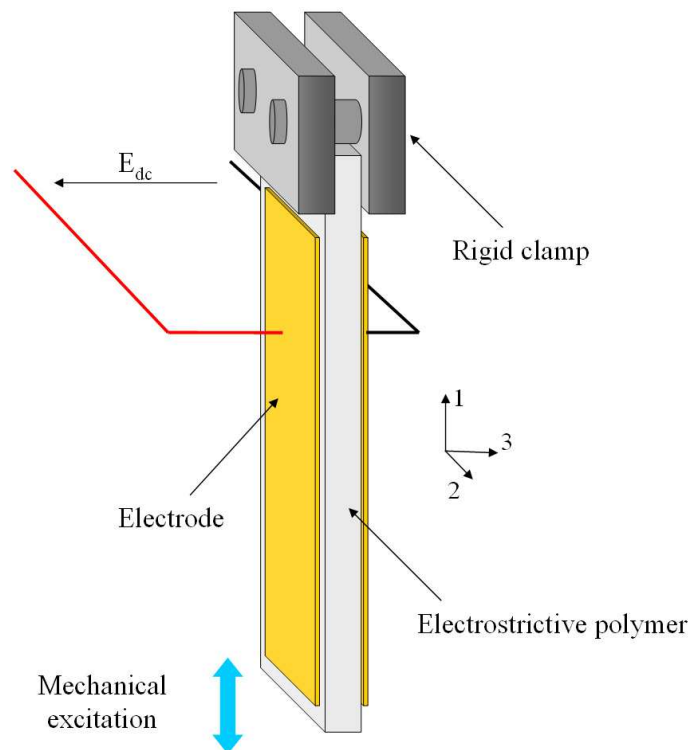
Fig. 3. Mechanical configuration of an electrostrictive polymer
