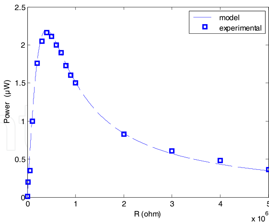
Fig. 11. The harvested power in AC for a constant electric field of 5\text{ V}/\mu\text{m} and a strain of 0.2\% at 100\text{ Hz} .
