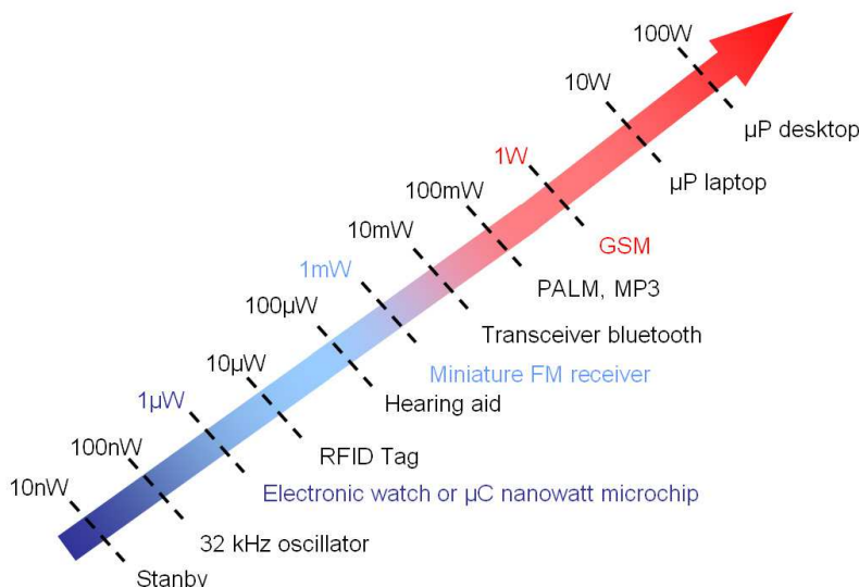
Fig. 13. The various powers consumed by CMOS electronic devices (Sebald, et al., 2008).
