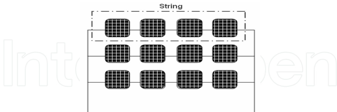
Fig. 12. PV generator configuration schematic
