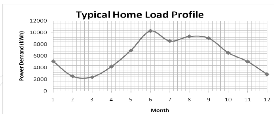
Fig. 3. Villa load profile in Al Ain (Source: AADC)
