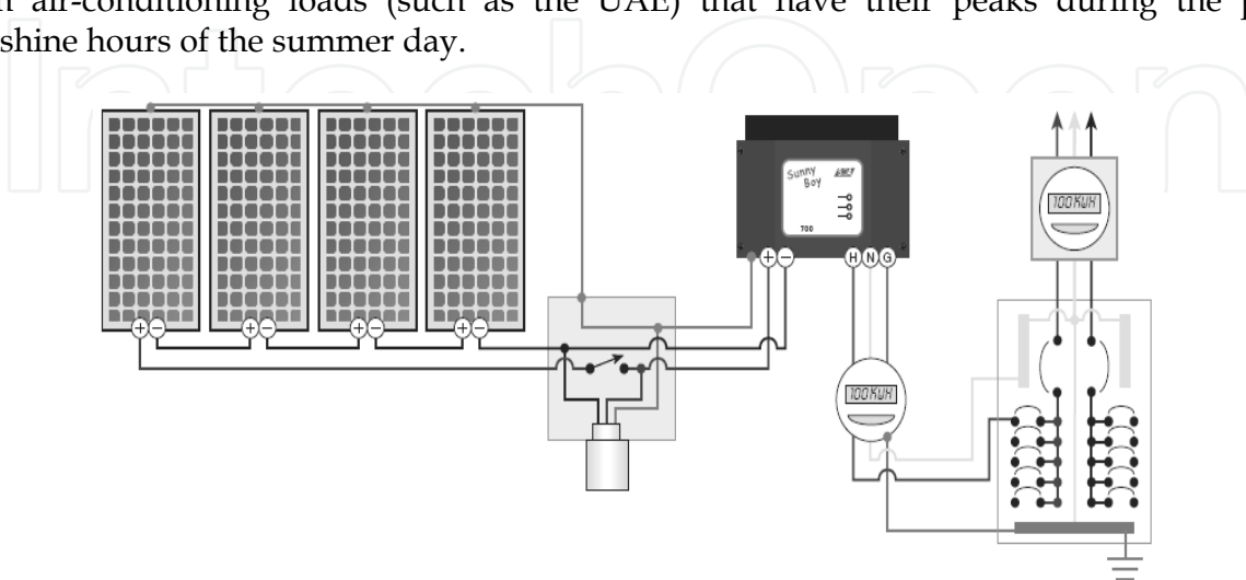
Fig. 2. Grid connected PV system schematic (source: www.homepower.com ),
