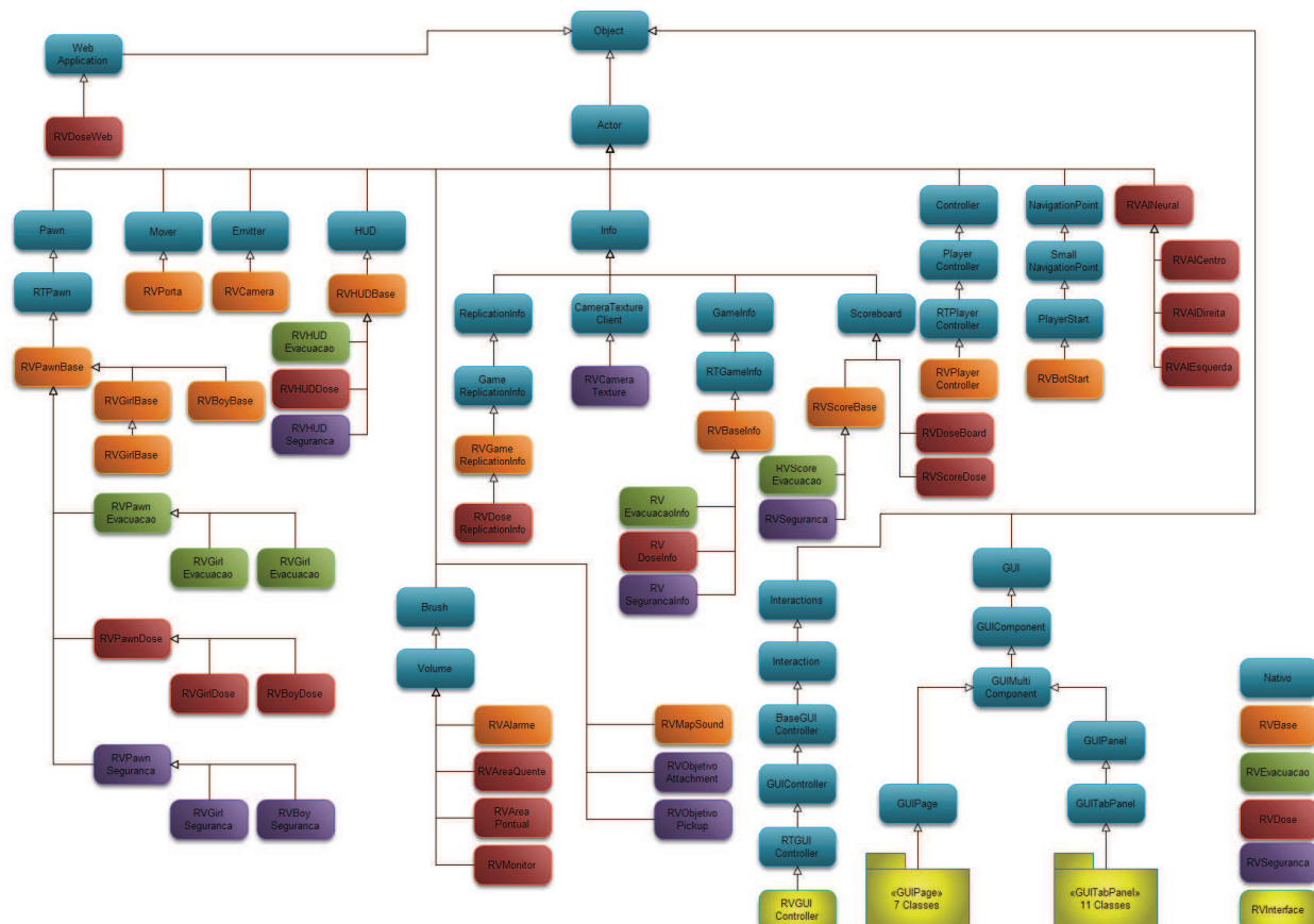
Fig. 1. Unreal Engine classes' structure
