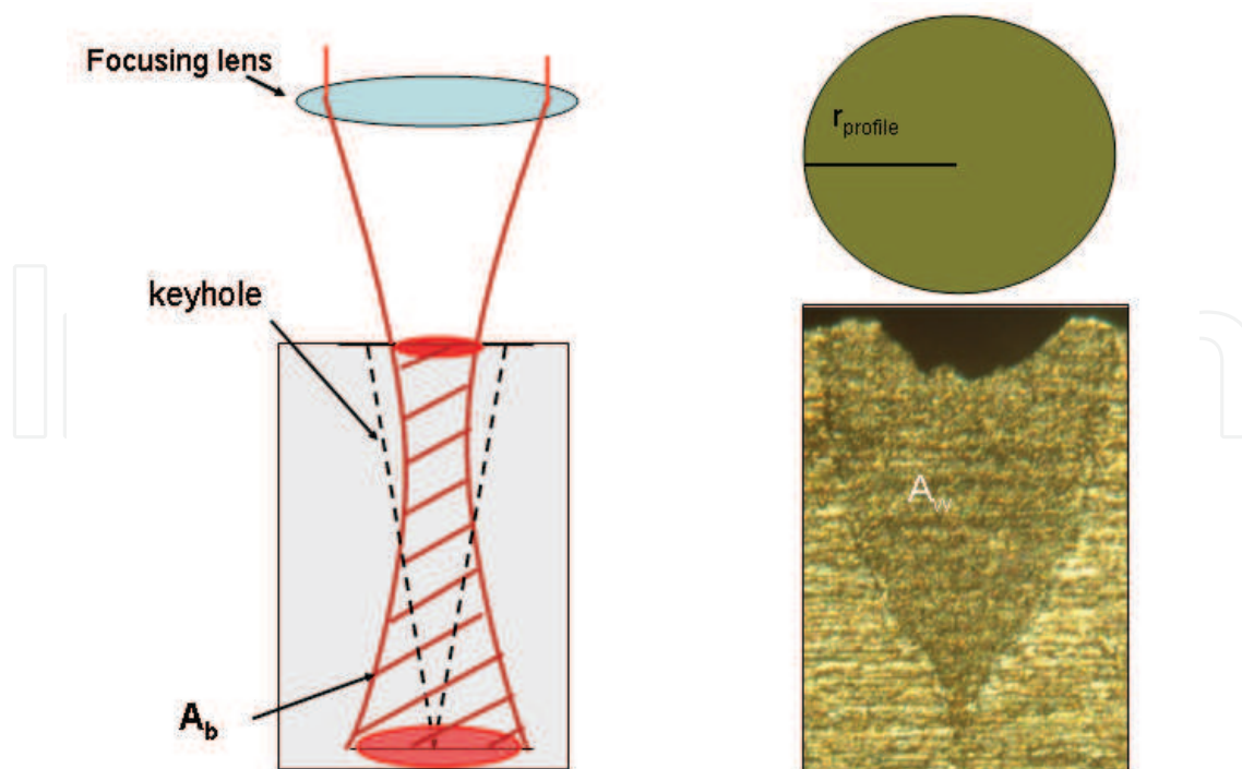
Fig. 7. Schematics showing the submerged beam surface area ( A_b ), the weld's cross-sectional area ( A_w ) and the profile radius ( r_{profile} )
