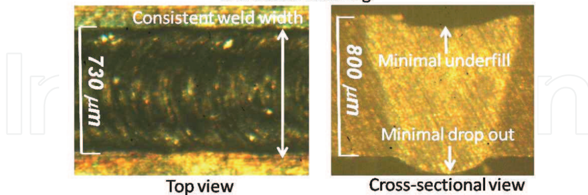
Fig. 14. Single-pass laser welded fatigue crack
