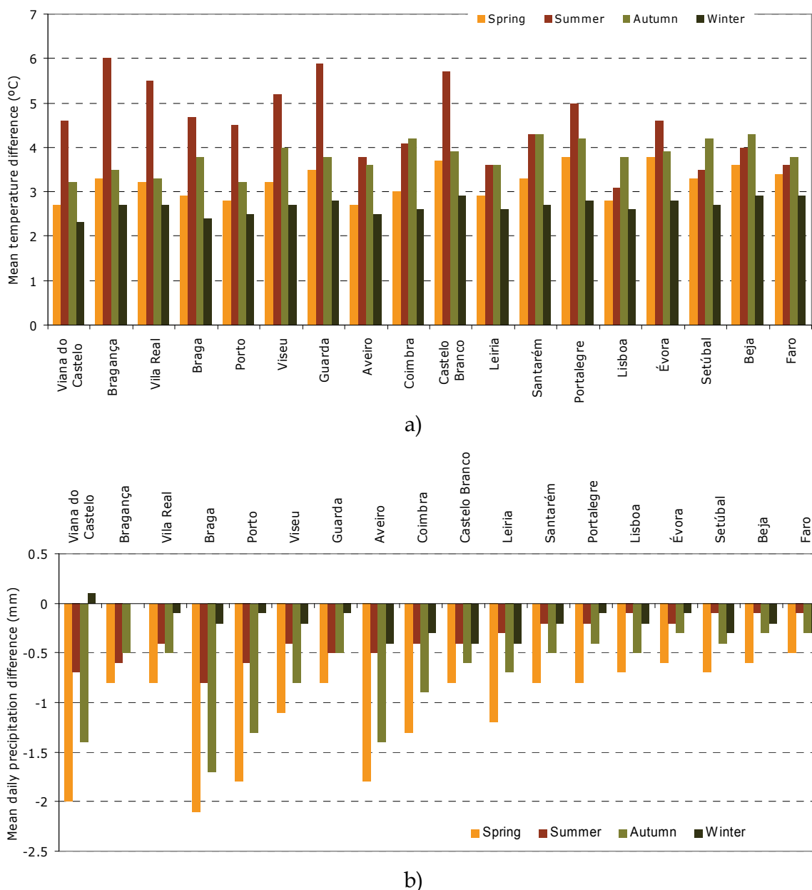
Fig. 6. Differences between future (2071-2100) and reference (1961-1990) climatic scenarios for a) daily mean temperature and b) daily precipitation, by season and for each Portuguese district.
