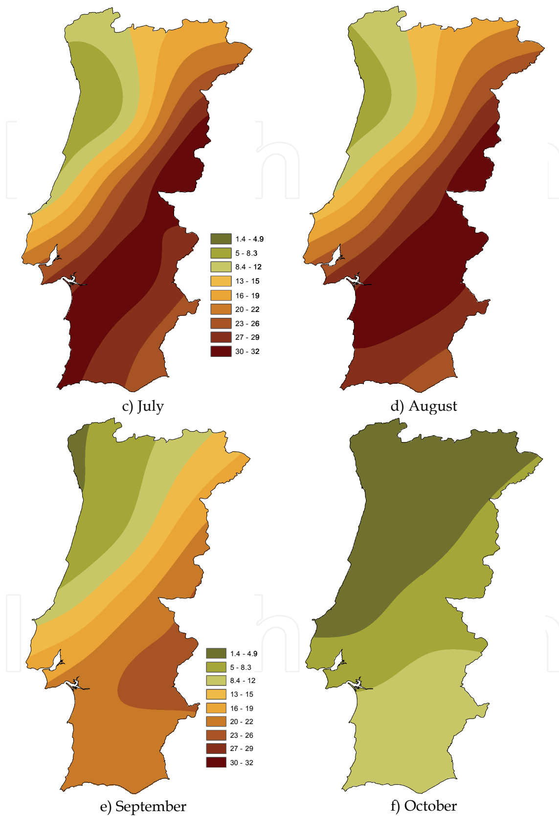
Fig. 5. Monthly mean fire weather index (FWI) between 1980 and 2005 for a) May, b) June, c) July, d) August, e) September, and f) October.
