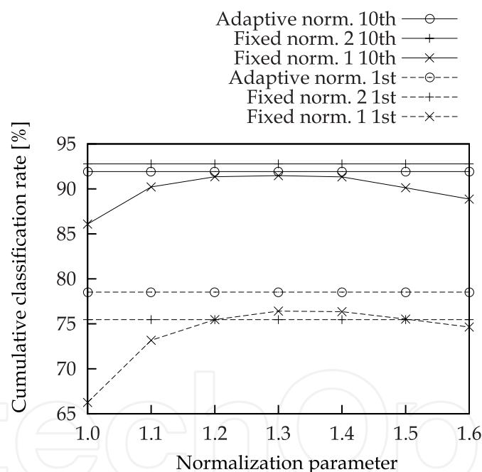
Fig. 8. Classification rates versus normalization parameter
