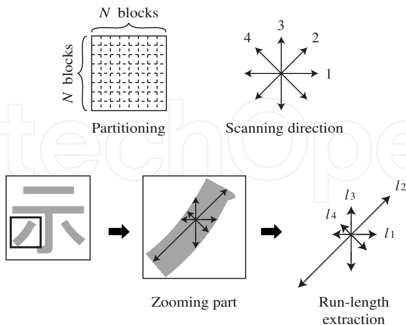
Fig. 2. Directional feature extraction.
