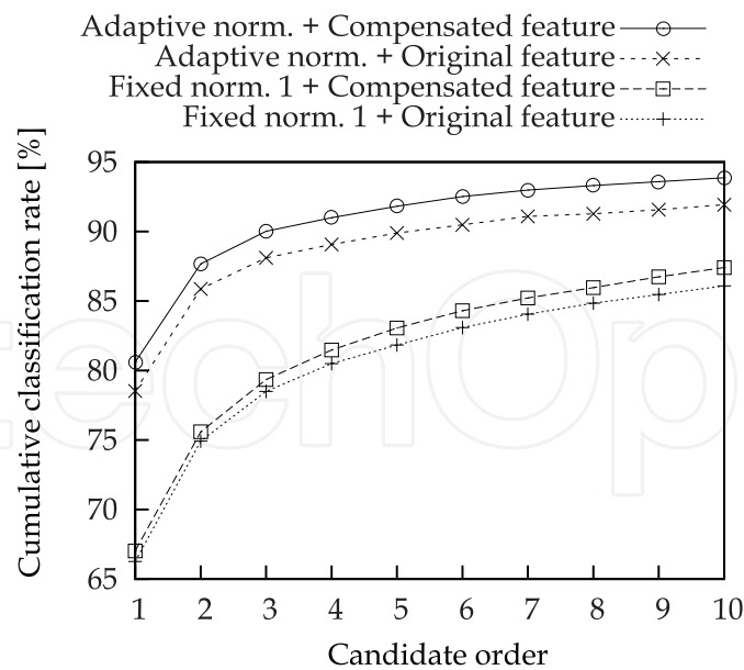
Fig. 10. Classification rates for all test data.
