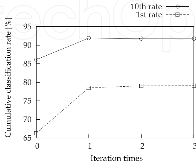
Fig. 11. Classification rates for each iteration time.
