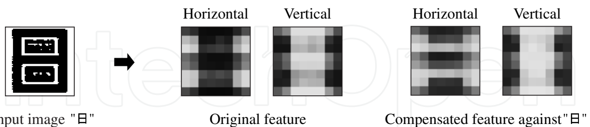
Fig. 6. Examples of feature values.
