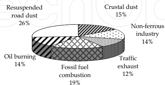
Fig. 5. PMF source contribution in bulk deposition
