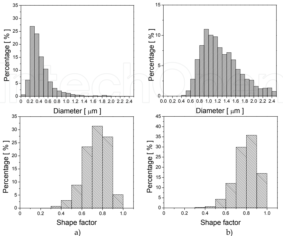
Fig. 8. Particle size distribution and shape factor of PM 2.5 samples in the a) non-heating and b) heating period.
