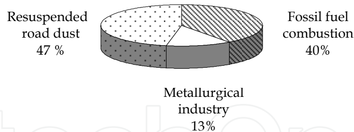
Fig. 2. Unmix resolved source contribution in PM 2.5
