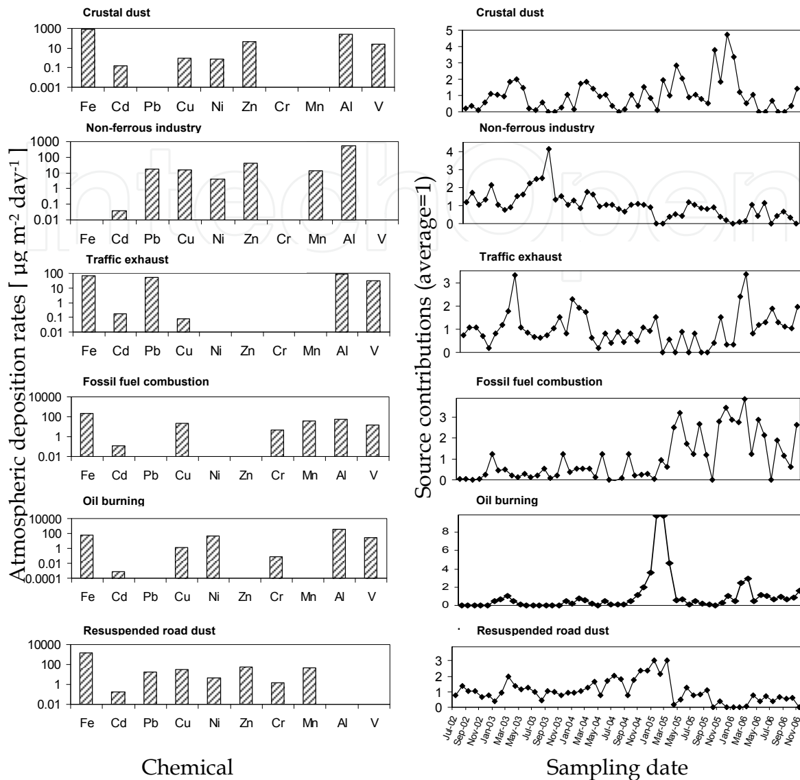
Fig. 4. Source profiles and time series plot of source contribution resolved from bulk deposition by PMF
