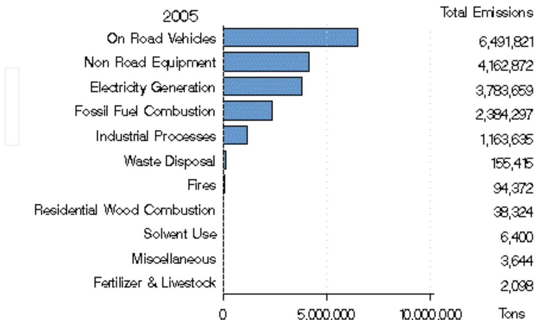
Fig. 6. USA emission sources of nitrogen oxides, 2005 (US EPA, 2009).
