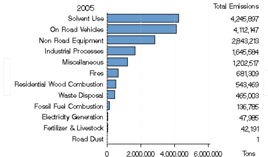
Fig. 17. USA emission sources of NMVOC, 2005 (US EPA, 2009).
