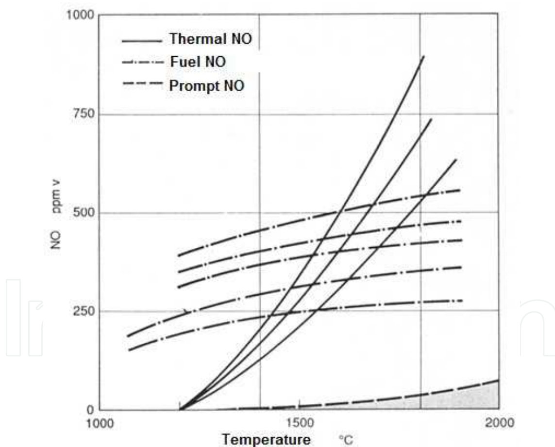
Fig. 8. Dependency between NO formation mechanisms and combustion temperature.
