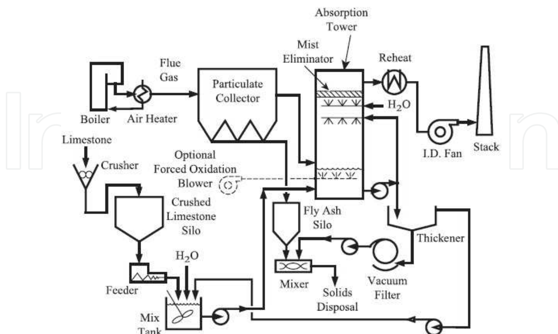
Fig. 18. Simplified wet limestone process flow diagram. (Schnelle & Brown, 2002)
