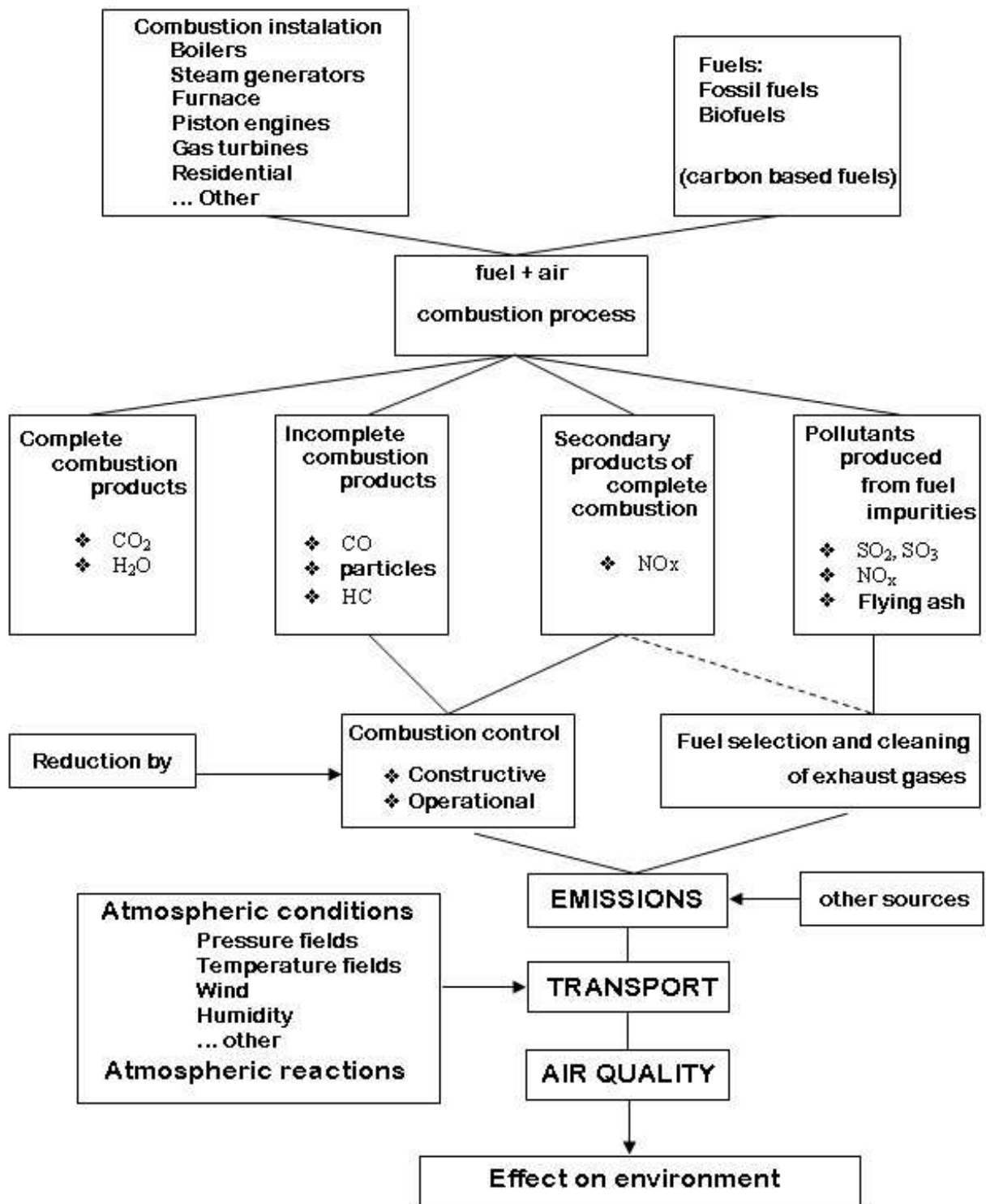
Fig. 1. Sources and products of anthropogenic pollution.
