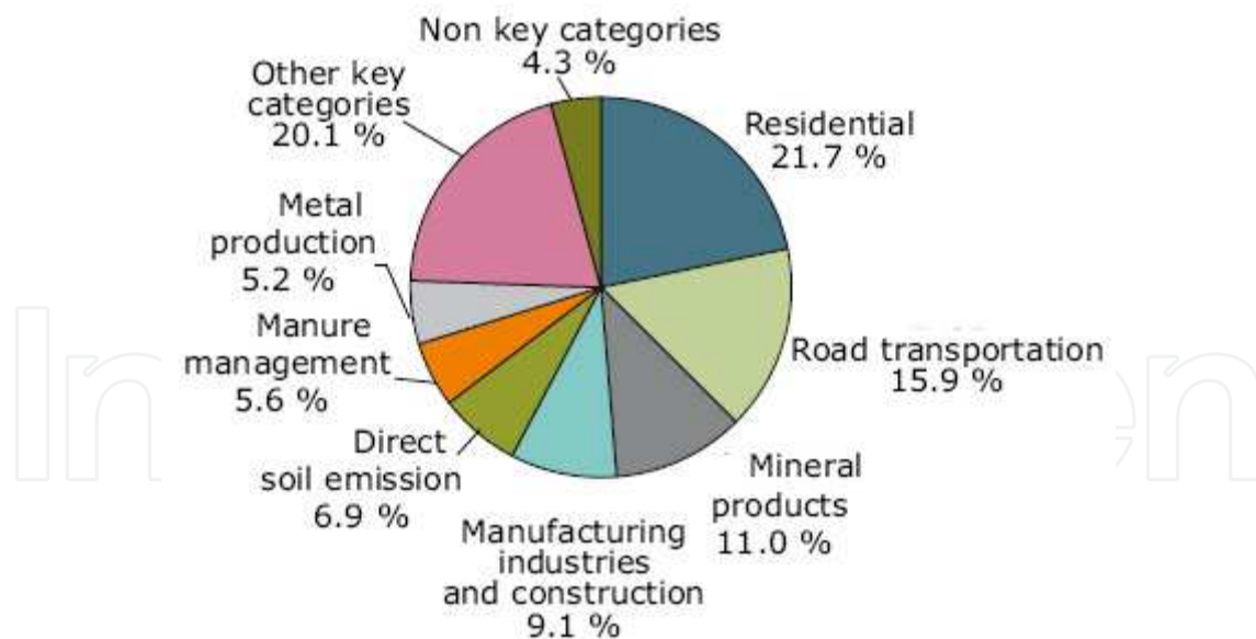
Fig. 12. EU-27 emission sources of PM10, 2006 (EEA, 2008).
