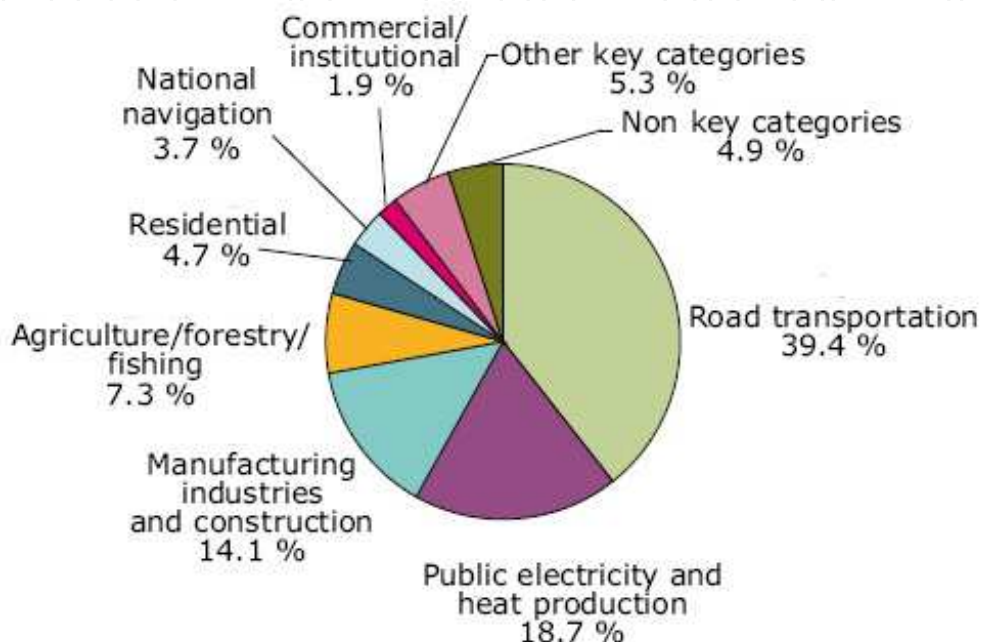
Fig. 5. EU-27 emission sources of nitrogen oxides, 2006 (EEA, 2008).
