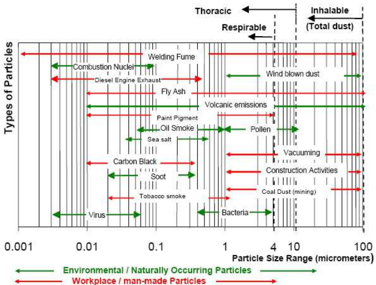
Fig. 14. Type of particles and their sources. (TSI, 2010)
