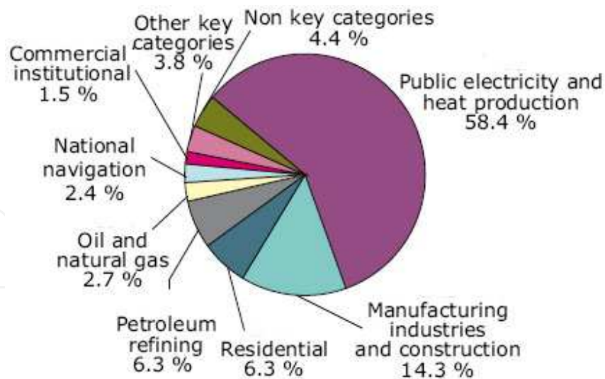
Fig. 9. EU-27 emission sources of sulphur oxides, 2006 (EEA, 2008).
