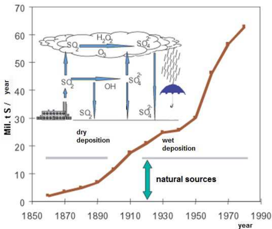
Fig. 11. SO_2 atmospheric reaction and historical emissions. (Popescu, 2009)
