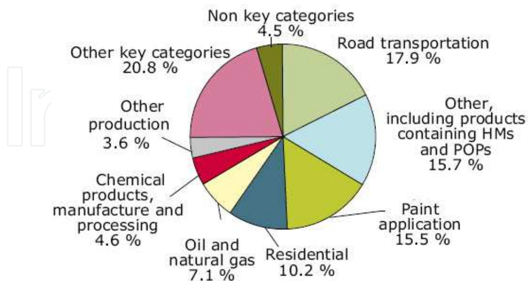
Fig. 16. EU-27 emission sources of NMVOC, 2006 (EEA, 2008).
