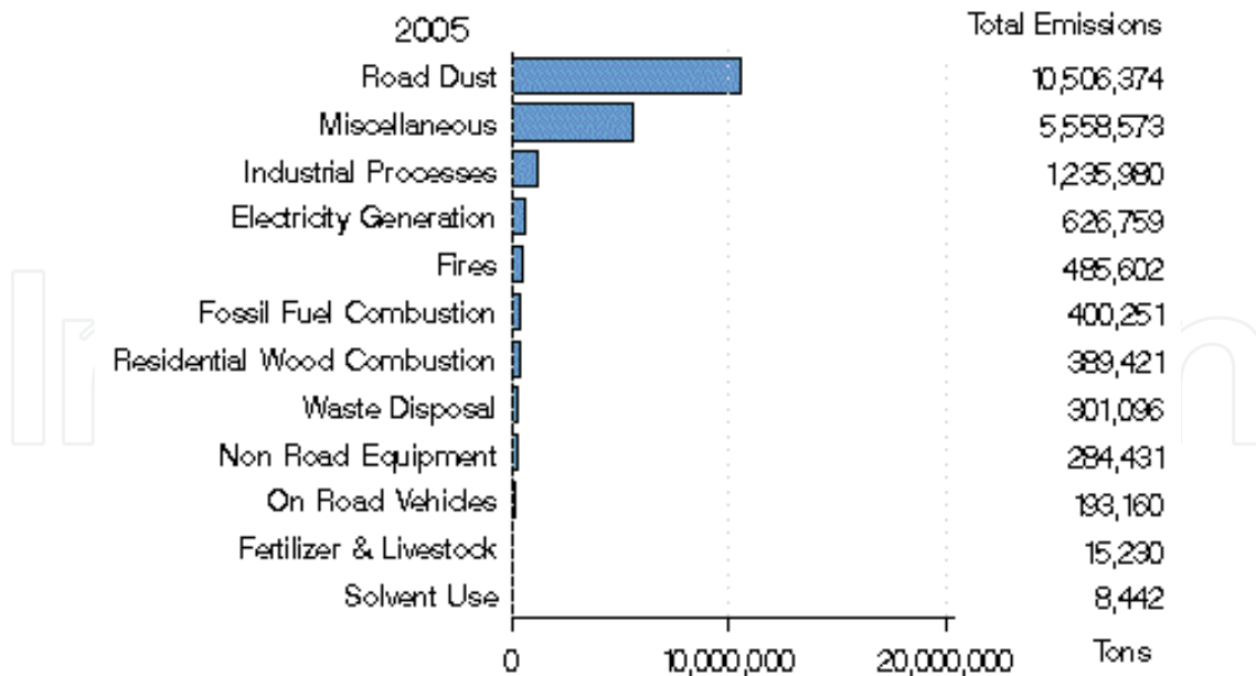
Fig. 13. USA emission sources of PM10, 2005 (US EPA, 2009).
