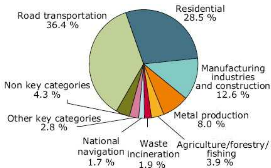
Fig. 3. EU-27 emission sources of carbon monoxide, 2006 (EEA, 2008).
