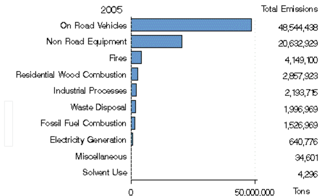
Fig. 4. USA emission sources of carbon monoxide, 2005 (US EPA, 2009).
