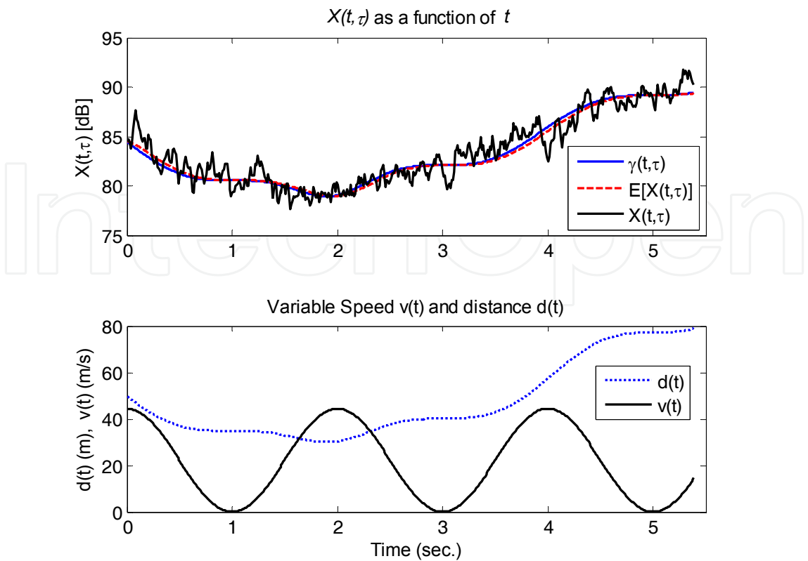
Fig. 3. Mean-reverting power path-loss X(t,\tau) for the TV LTF wireless channel model in Example 2.
