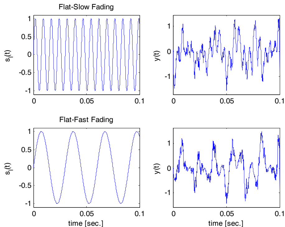
Fig. 9. Input signal, s_i(t) , and the corresponding received signal, y(t) , for flat slow fading (top) and flat fast fading conditions (bottom).
