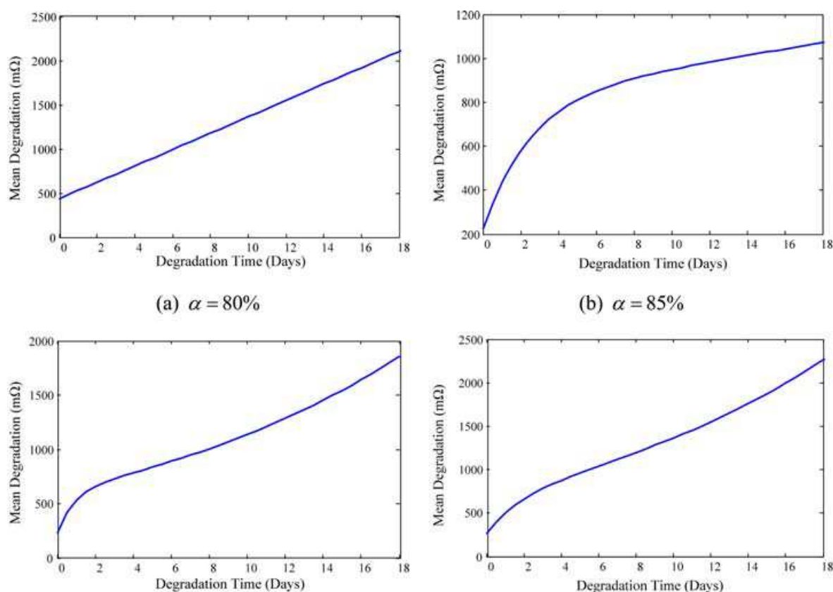
Fig. 5. Mean degradation value of contact resistance versus time for joints with various cure degree
