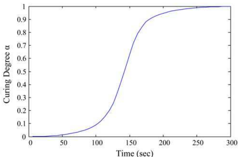
Fig. 8. ACF curing degree versus time under constant heating rate ( 20^{\circ}\text{C}\cdot\text{min}^{-1} )
