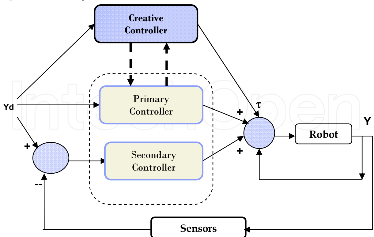
Fig. 4. Block diagram of creative controller
