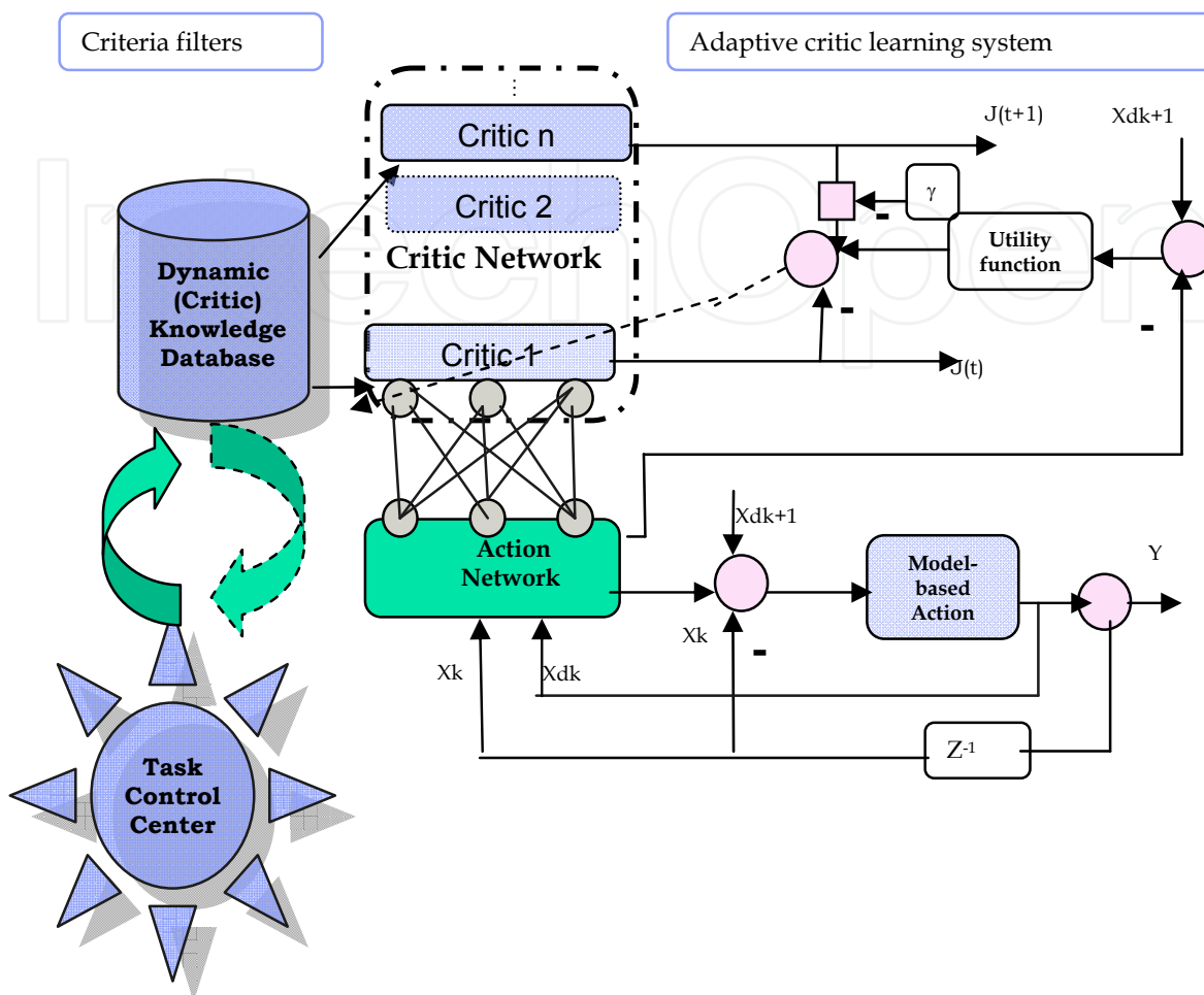
Fig. 2. Proposed Creative Learning Algorithm Structure
