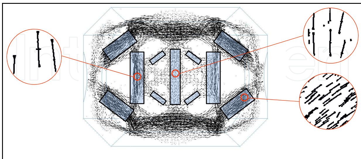
Fig. 15. Principle stress highlighted for a laminate.
