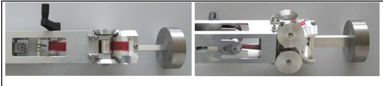
Fig. 12. Functional prototype.
