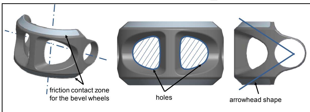
Fig. 16. 3D-CAD model of a design proposal.
