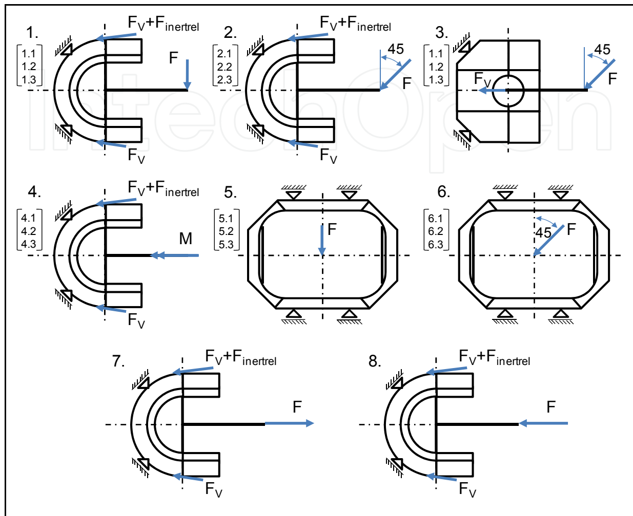
Fig. 13. Load cases for the topology optimization.
