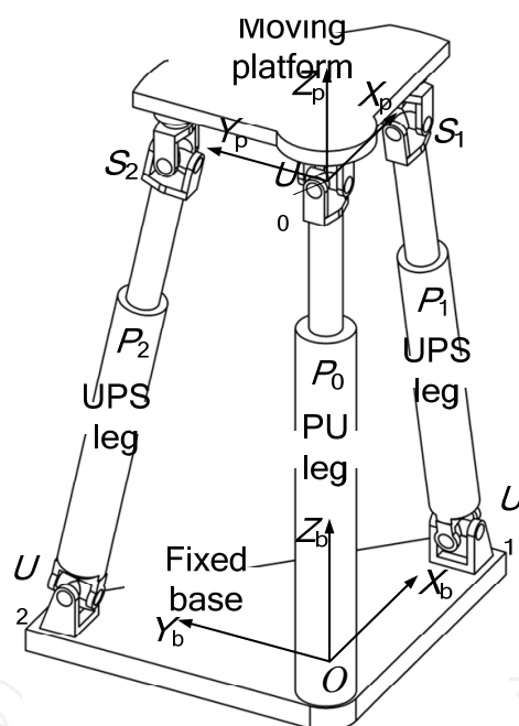
Fig. 1. The 2-UPS-PU parallel manipulator
