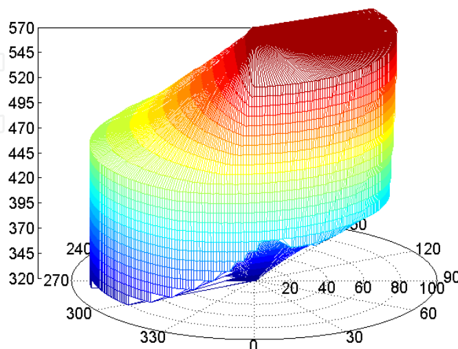
Fig. 5. Isometric view of the Parallel manipulator's workspace.
