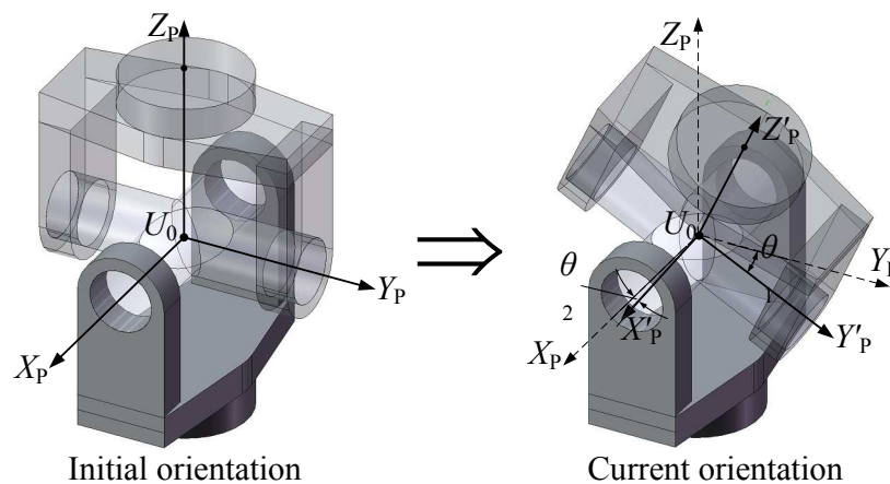
Fig. 2. The 2-UPS-PU parallel manipulator
