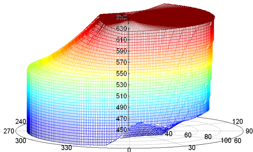
Fig. 8. Isometric view of the Parallel manipulator's workspace.
