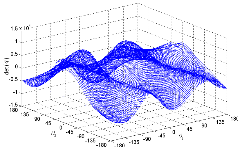
Fig. 3. The relationship between the determinant of jacobian matrix and \theta_1 , \theta_2
