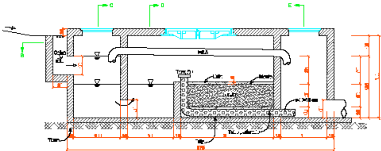
Fig. 6. Design of Guerengue sand filter
