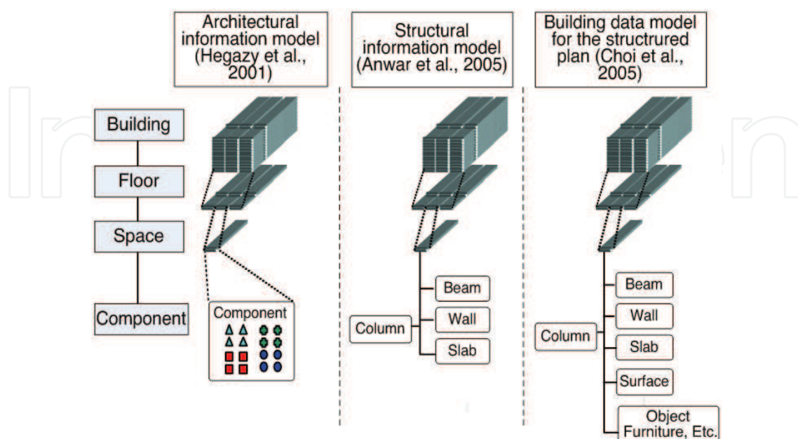
Fig. 4. Building project hierarchy according to the building information model
