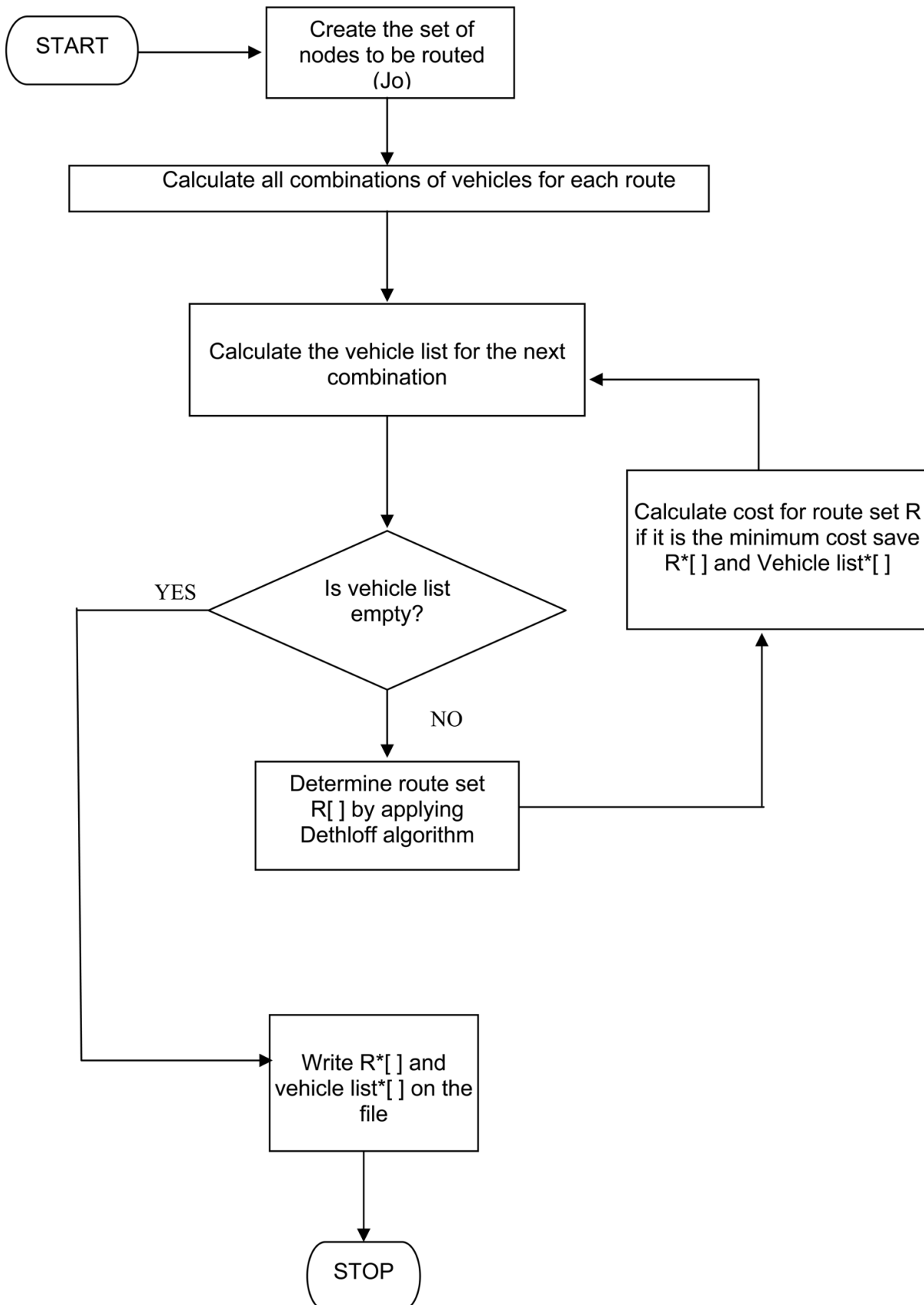
Fig. 6. Flowchart of proposed algorithm
