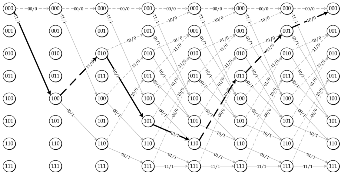
Fig. 4. Decoder trellis diagram showing the path for the input codeword of 11111010101110.
