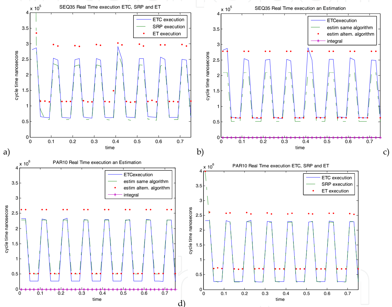
Fig. 9. Real Time Execution of the ETC with a sequential SFC of 35 states and a concurrent SFC compound of 10 sequential SFCs.
