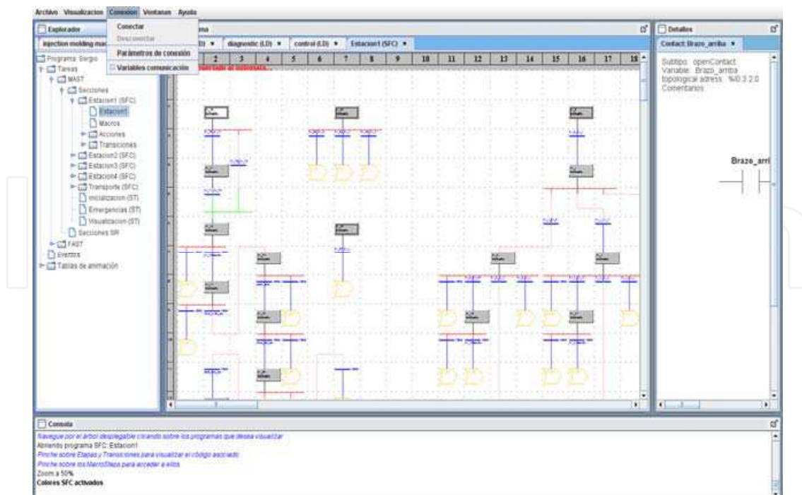
Fig. 2. PLC programming in Sequential Function Chart
