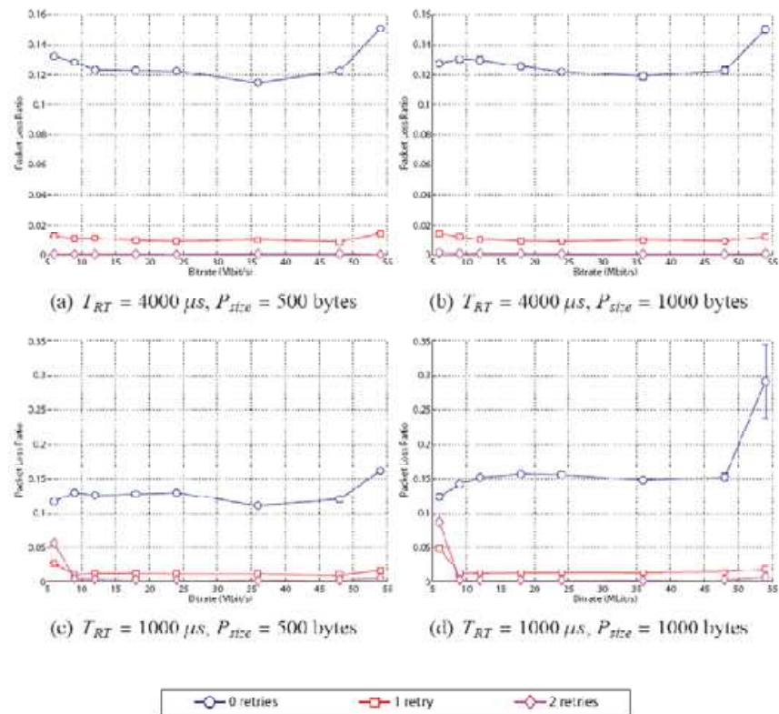
Fig. 12. Packet Loss Rate.
