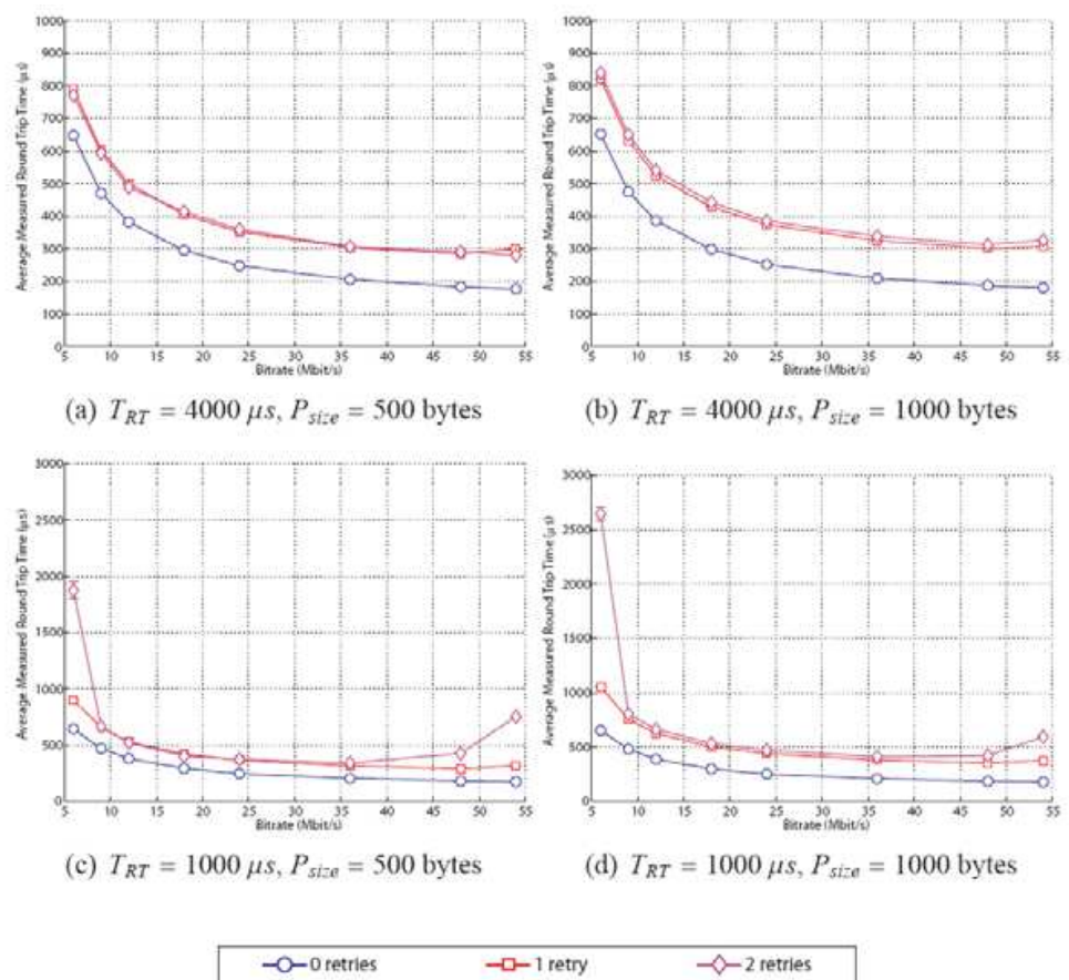
Fig. 11. Average measured Round Trip Time.
