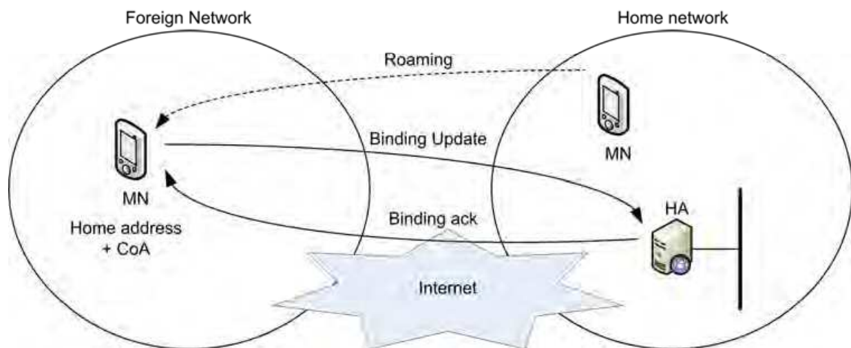
Fig. 3. MIPv6 Operation
