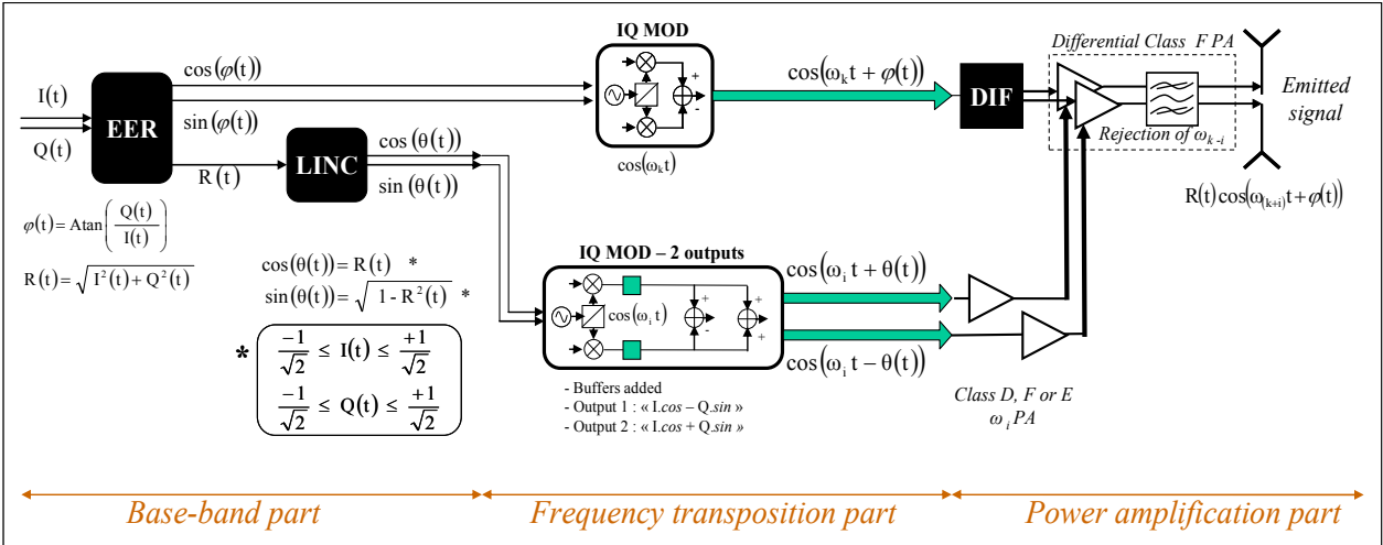
Fig. 14. EER-LINC method for high PAPR signals
