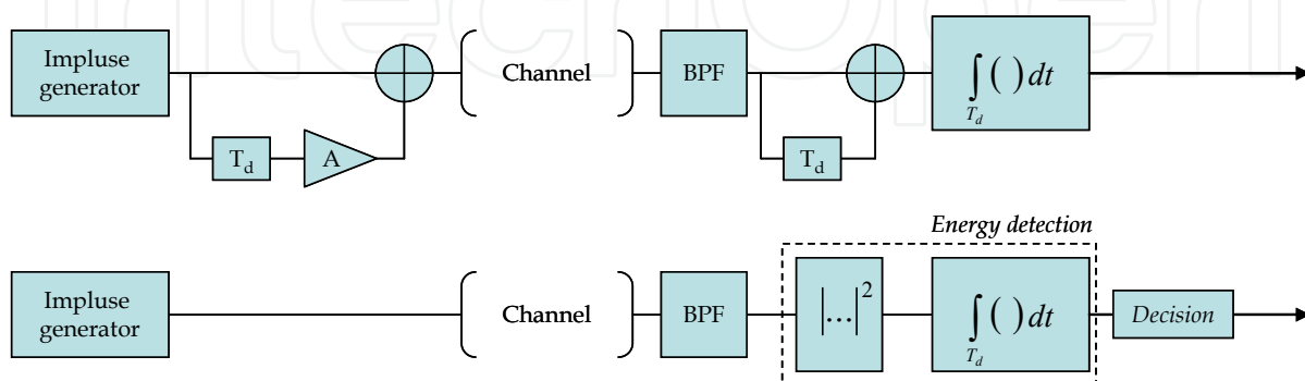
Fig. 28. Examples of NCo-Rx transmitter and receiver
