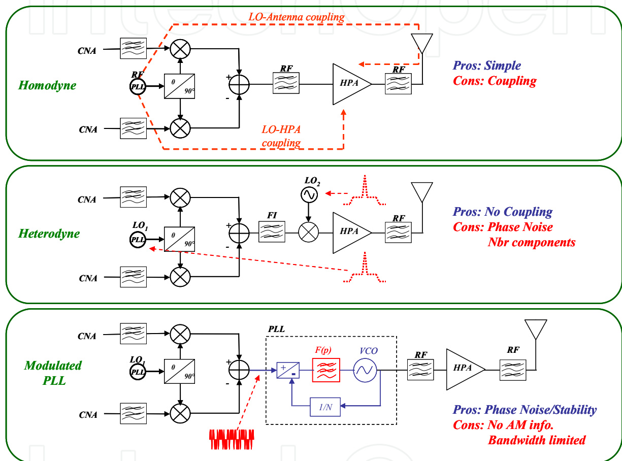
Fig. 9. Classic architectures for RF transmitters
