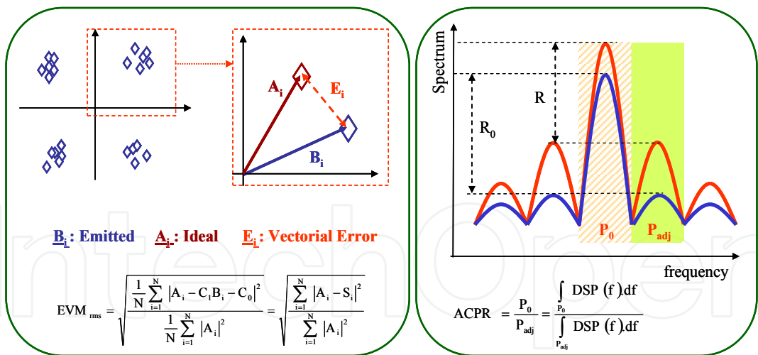
Fig. 3. EVM and ACPR definitions
