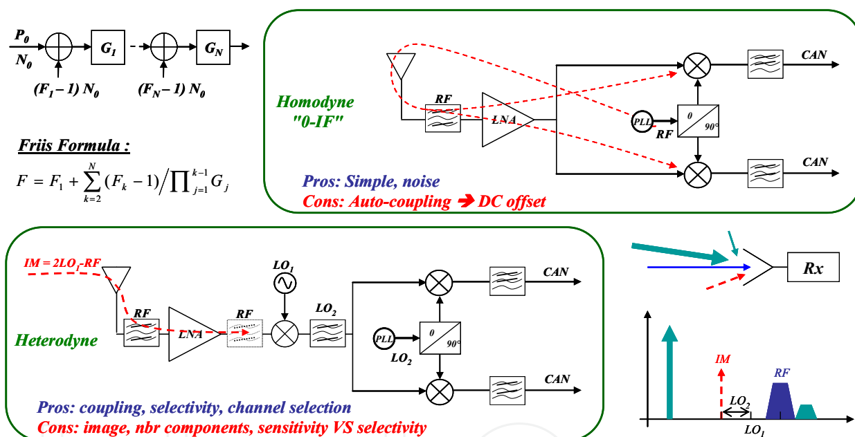
Fig. 15. Considerations for receiver architectures
