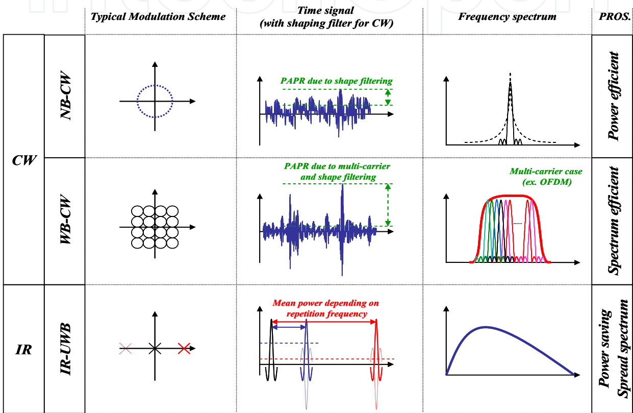
Fig. 1. Main types of radio-communications signals
