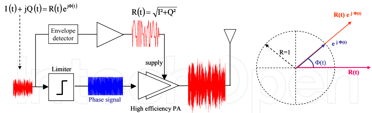
Fig. 12. Principle of the EER technique [Kahn, 1952]
