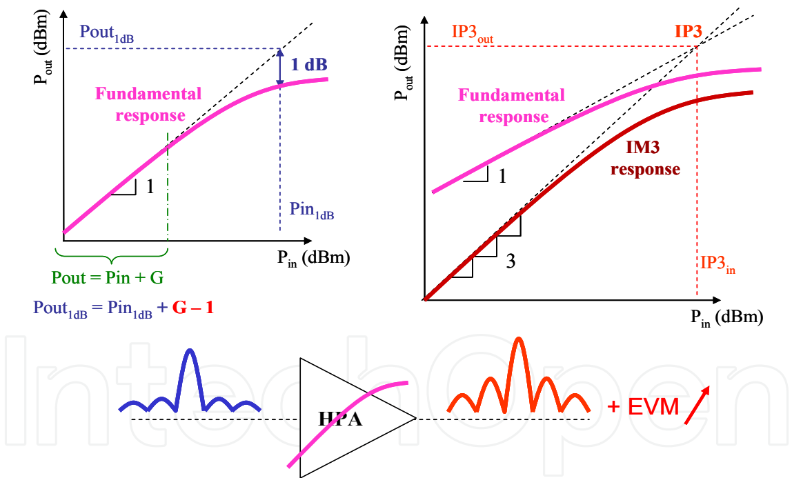
Fig. 7. Compression effect modeling for 1 ton (P1dB) and 2 tons (IP3)
