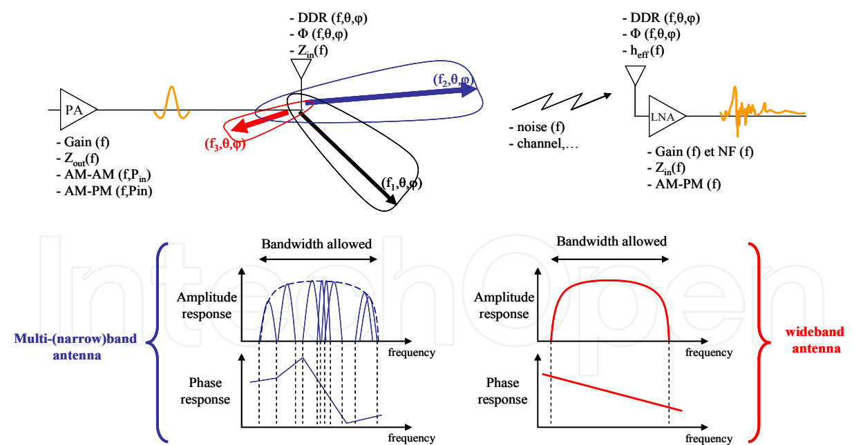
Fig. 8. Antenna system characteristics in radio-communications
