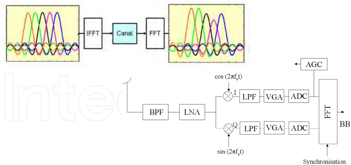
Fig. 29. Considerations for MB-OFDM UWB transceivers
