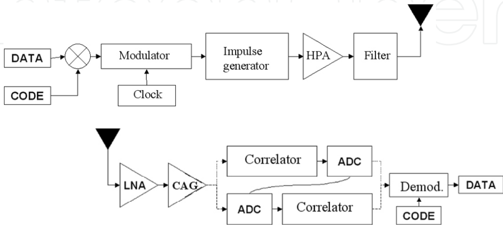
Fig. 27. Examples of Co-Rx transmitter and receiver
