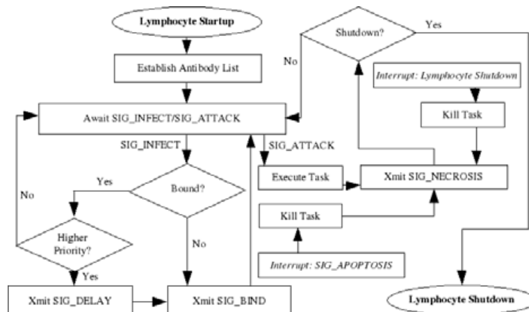
Fig. 4. Control flow graph of lymphocytic agent
