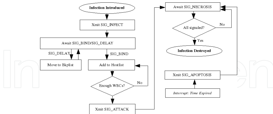
Fig. 3. Control flow graph of infectious agent
