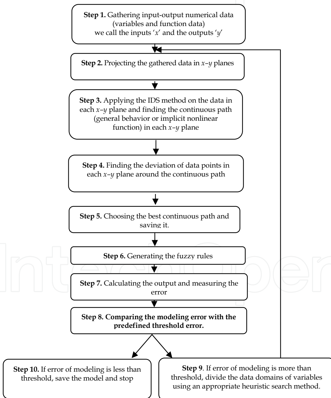
Fig. 1. Proposed algorithm for Active Learning Method.
