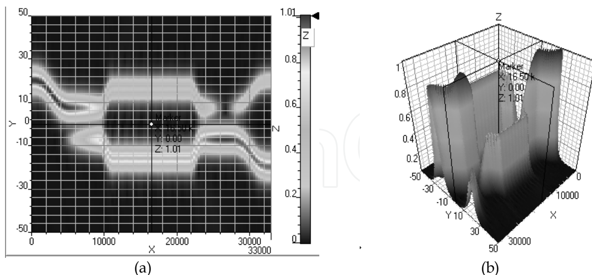
Fig. 4. (a) Switch with CROSS state (b) Optical field propagation for CROSS state (3D View)
