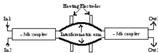
Fig. 2. Basic 2x2 MZI switch structure, ref. [10]
