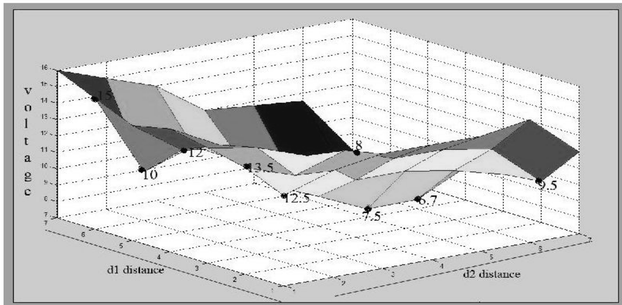
Fig. 8. Graphical (3D view) representation of the switching voltage v/s d_1 & d_2
