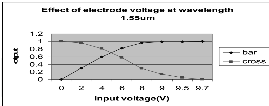
Fig. 10. Variation of output power with electrode voltage ( \lambda=1.55 \mu\text{m} )
