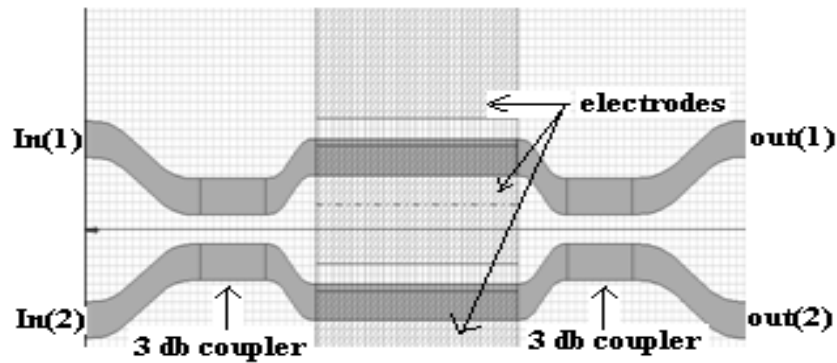
Fig. 3. 2 x 2 MZI switch layout
