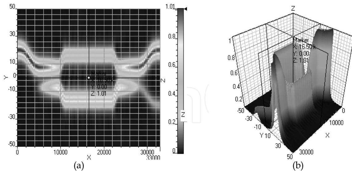
Fig. 5. (a) Switch with BAR state (b) Optical field propagation for BAR state (3D view)
