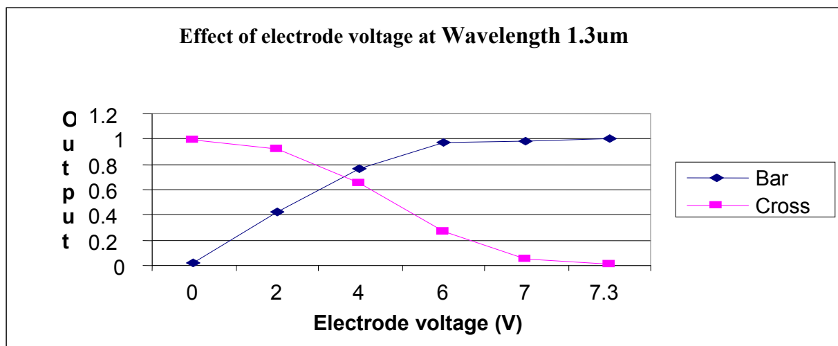
Fig. 9. Variation of output power with electrode voltage ( \lambda=1.3 \mu\text{m} )
