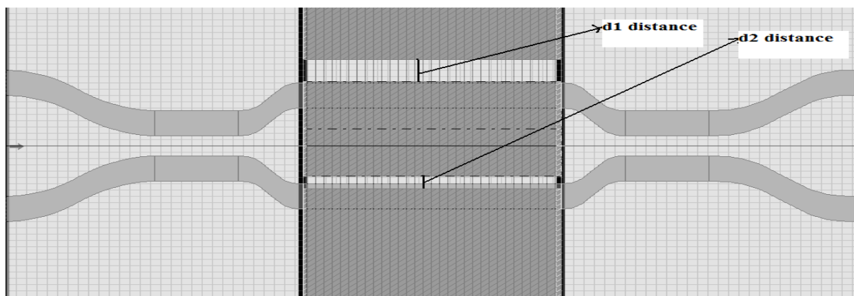
Fig. 6. Layout of the MZI switch with parameters given above.
