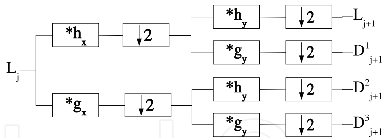
Fig. 3. 2D DWT using FIR filters
