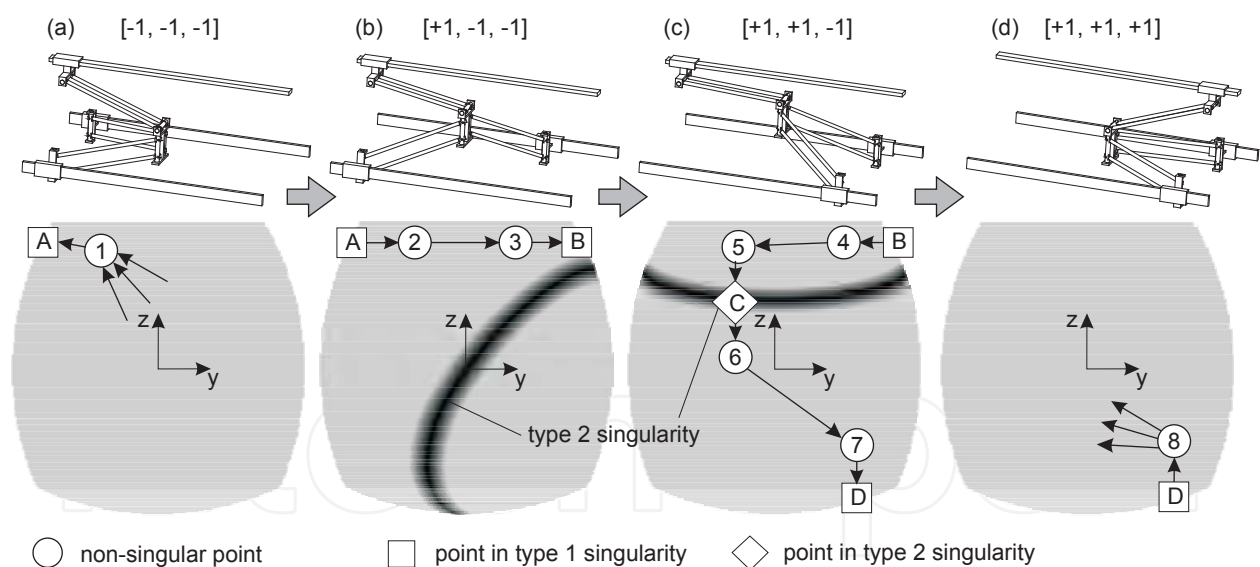
Fig. 5. Changing the working configuration
