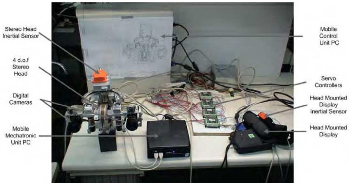
Fig. 1. The Stereo vision system.
