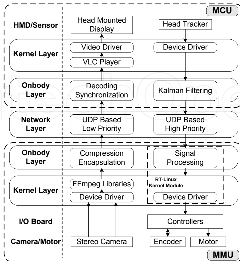
Fig. 3. Flowchart of the stereo vision software architecture.
