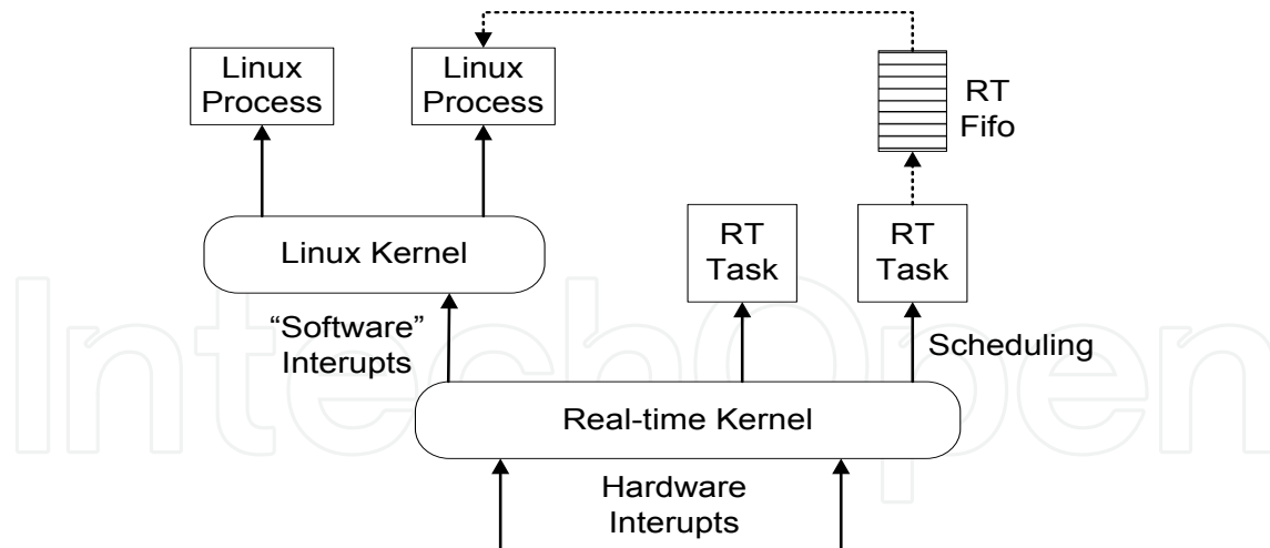
Fig. 4. The chosen operating system combines the use of two kernels, RT-Linux and Linux to provide support for critical tasks and soft real-time applications, respectively.
