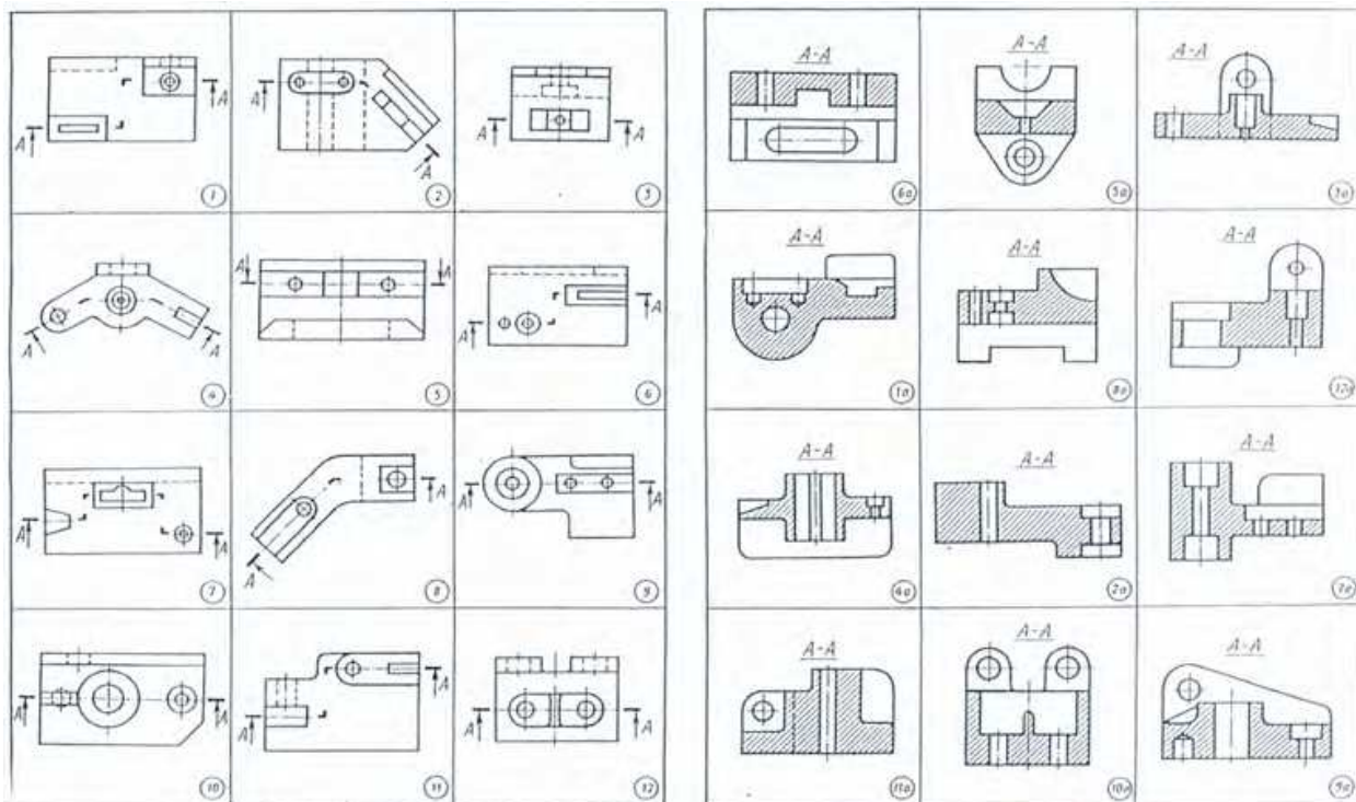
Fig. 38. Example of cutting fast exercise, the student must link the cutting plane and the cutting view [19]
