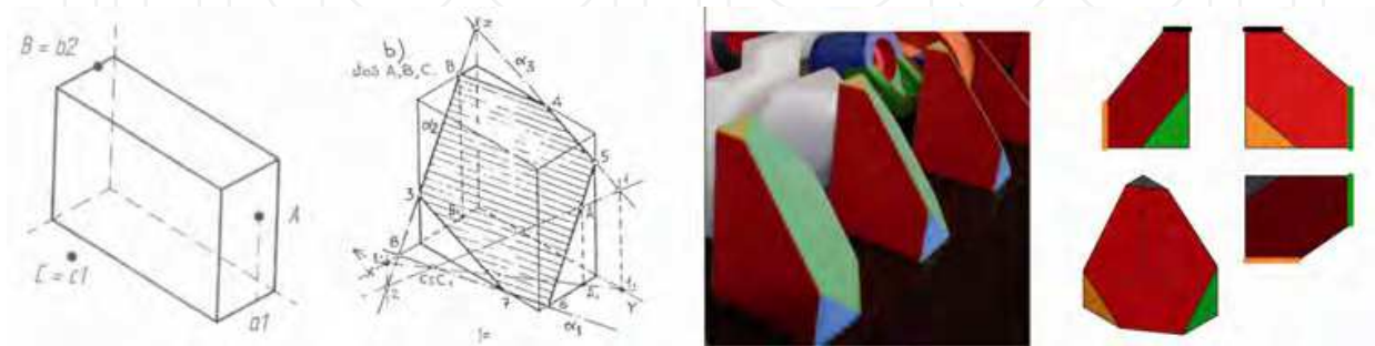
Fig. 34. Box-plane intersections exercise, solution, models and CAD views
