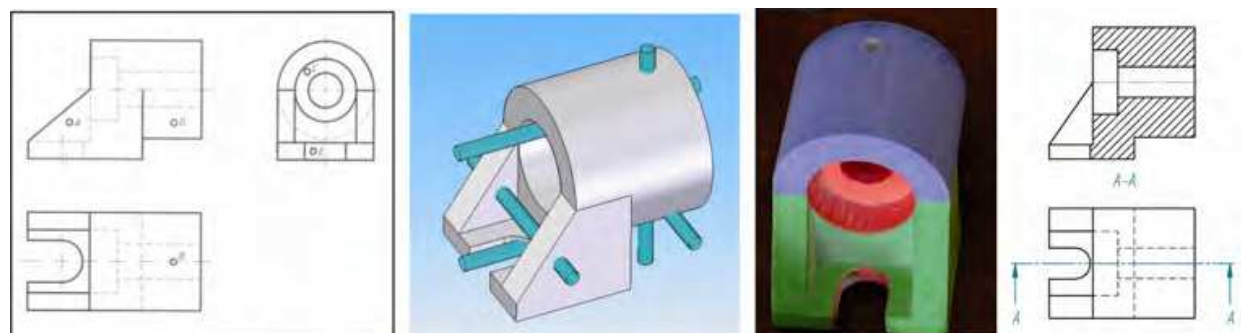
Fig. 37. Example of drilling exercises [20] (student must know when there is material and when there is vacuum) and CAD, physics model and cutting view
