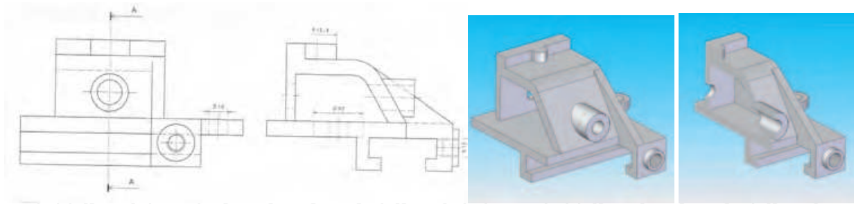
Fig. 40. Example of exercise with intersections between surfaces and CAD models
