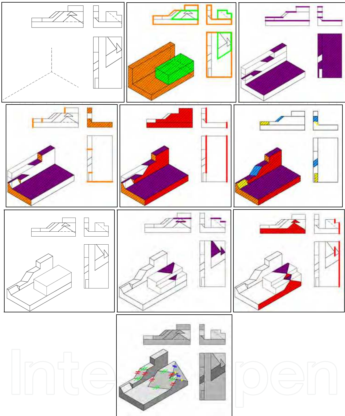
Fig. 35. Example of flat piece resolution process
