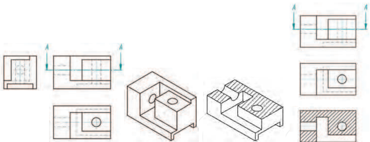
Fig. 39. Example of simple cutting exercise
