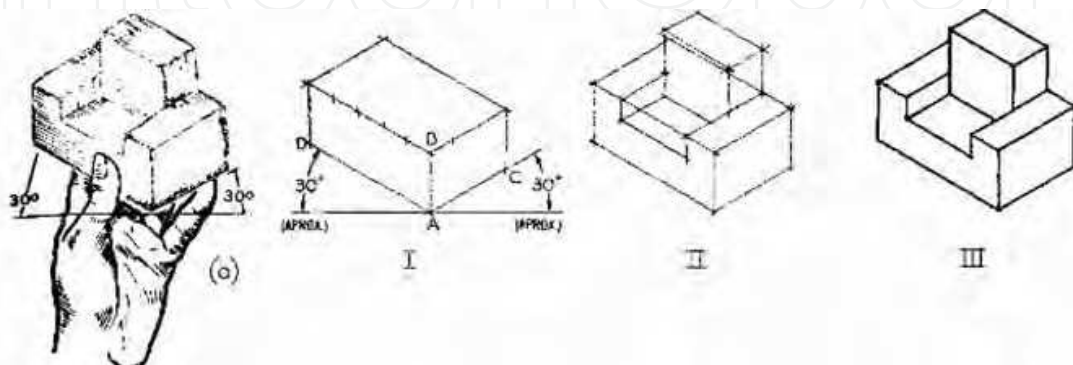
Fig. 18. Sketching process [15]
