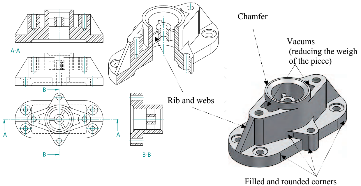
Fig. 16. Piece with several industry's characteristic features
