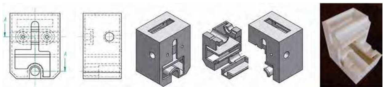
Fig. 42. Exercises with high level of spatial Visualization, CAD and physics model
