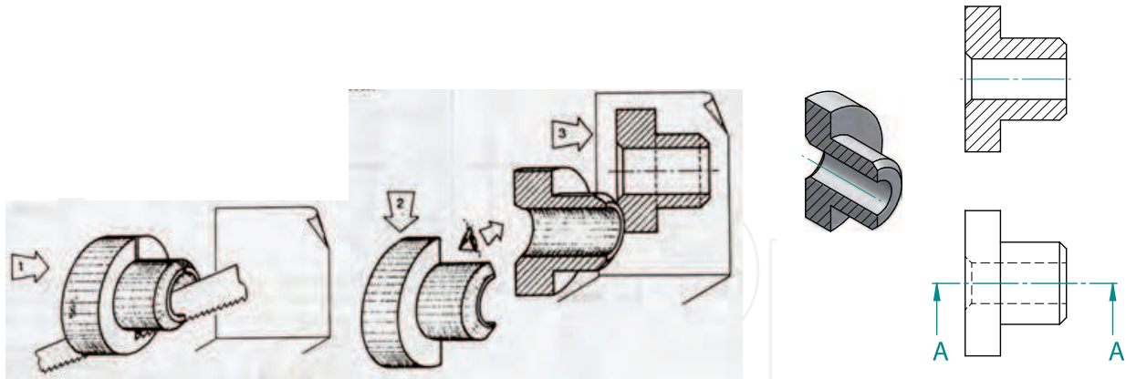
Fig. 14. cutting plane
