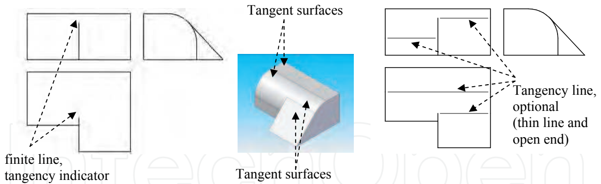
Fig. 11. Tangent surfaces and tangency line
