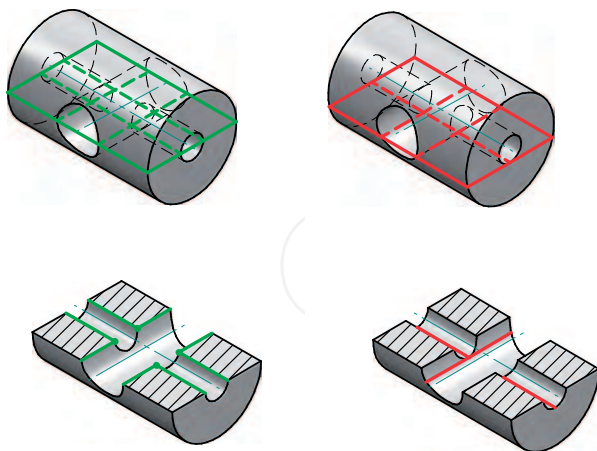
Fig. 19. Cylinder intersection sketching process
