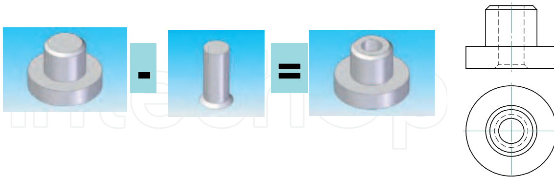
Fig. 13. Vacuum = material (+) - material (-). The vacuum is always surrounded by material
