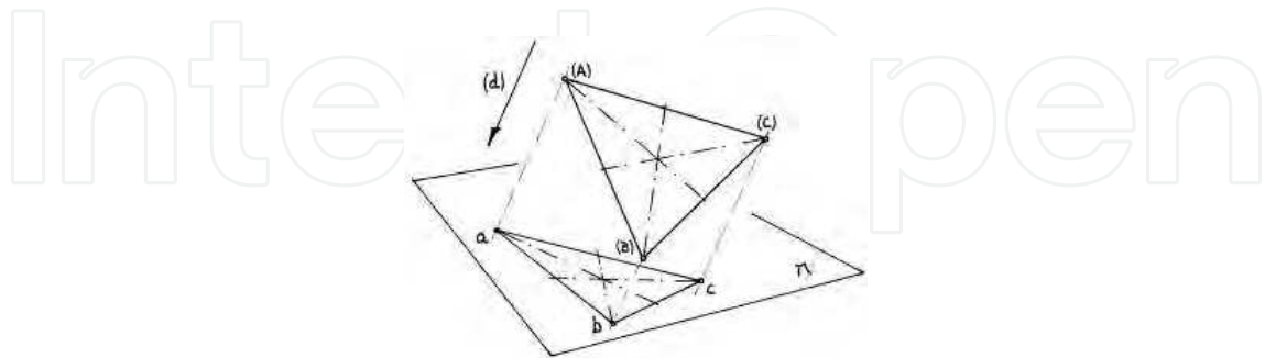
Fig. 7. The form of flat surfaces remains equal but the dimensions are not in true scale unless the feature is parallel to the projection plane
