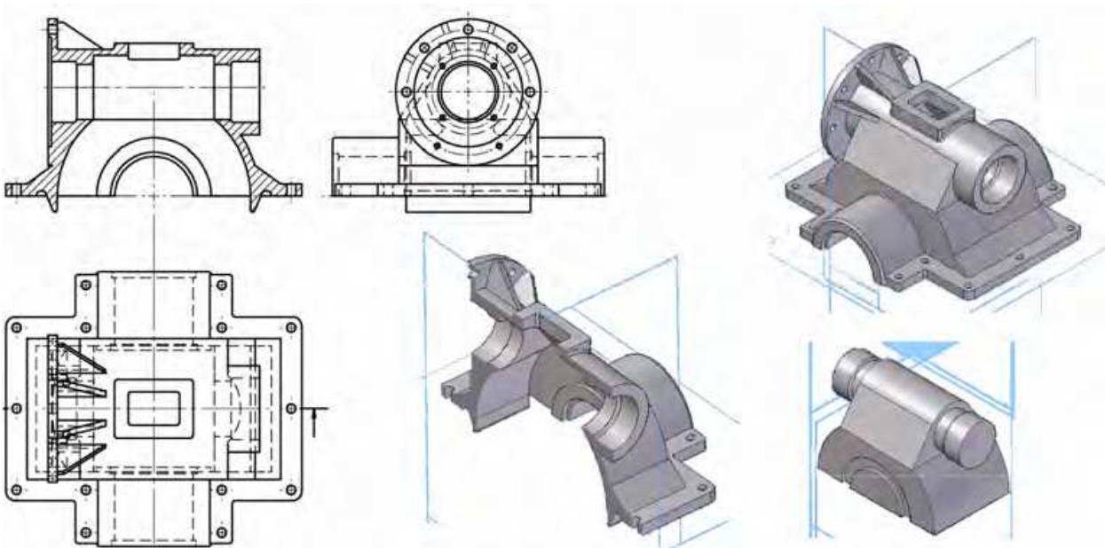
Fig. 43. Exercise with industrial features, intersection and tangency between surfaces and negative elements (vacuum)
