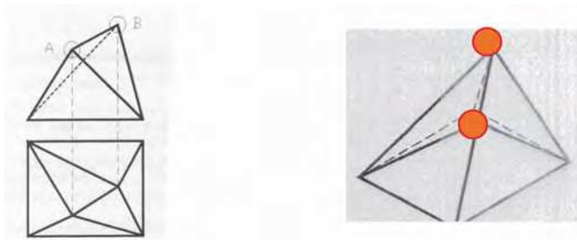
Fig. 22. First steps of solving process, identifying the planes which are parallel to the projection planes
