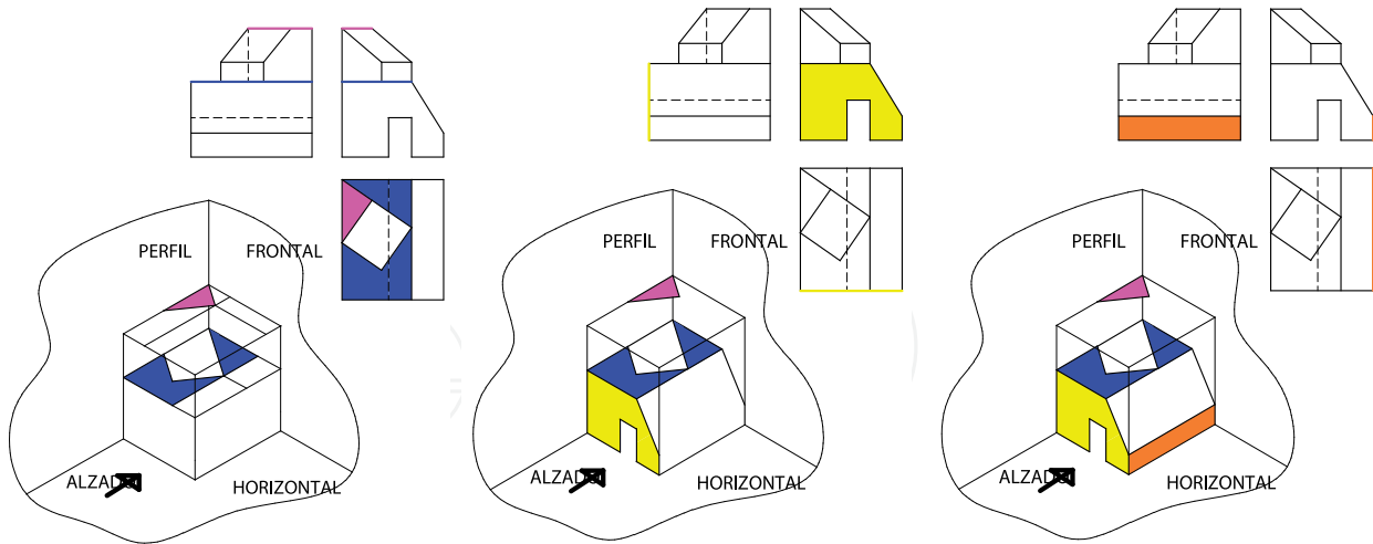
Fig. 22. First steps of solving process, identifying the planes which are parallel to the projection planes
