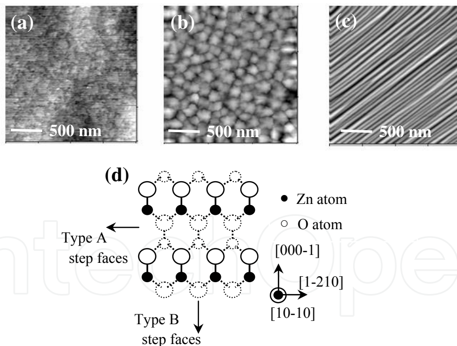
Fig. 2. AFM images of Zn-polar (a), O-polar (b) and M -nonpolar (c) ZnO layer surfaces. (d) Structural models showing the M -nonpolar (10-10) surfaces of ZnO.
