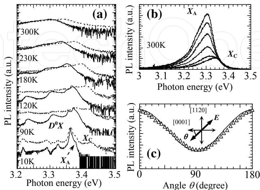
Fig. 15. (a) Temperature dependence of PL spectra on strain-free ZnO layers for E_{\perp}c (solid lines) and E//c (dotted lines). (b) Polarization-dependent PL spectra at 300 K taken in steps of \Delta\theta = 15^\circ . (c) PL intensity as a function of polarization angle \theta . Inset shows a schematic representation of the measurement geometry and sample orientation
