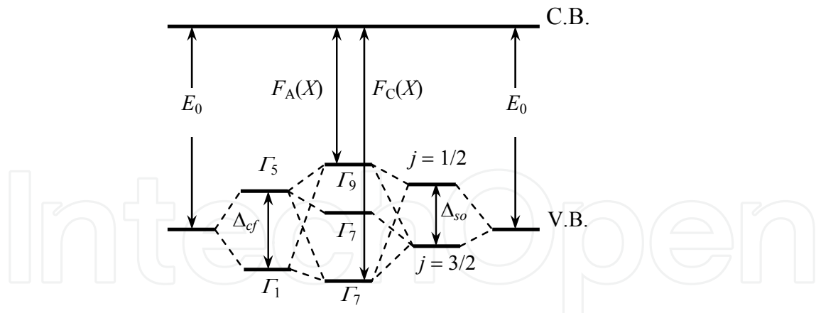
Fig. 14. Schematic energy level of band splitting by the crystal-field ( \Delta_{cf} ) and spin-orbit ( \Delta_{so} ) interactions in a wurtzite structure. F_A(X) and F_C(X) correspond to A and C-excitons, respectively, which are indicated in the middle. In the electronic energy levels proposed by Park et al. and Reynolds et al. , the uppermost \Gamma_9 and \Gamma_7 levels are interchanged.
