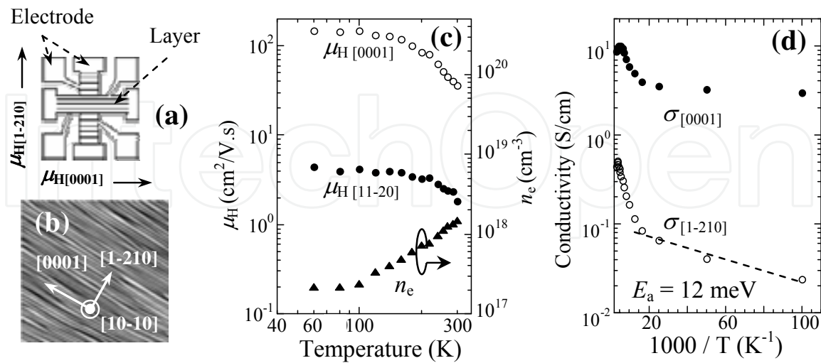
Fig. 17. (a) Hall bar patterned used to investigate anisotropic transport. (b) An AFM image of the Mg 0.12 Zn 0.88 O/ZnO MQWs. (c) Temperature dependence of \mu_{H[0001]} and \mu_{H[1-210]} for MQWs with a L_W of 2.8 nm. (d) Temperature dependence of \sigma_{[0001]} and \sigma_{[1-210]} for MQWs with a L_W of 2.8 nm.
