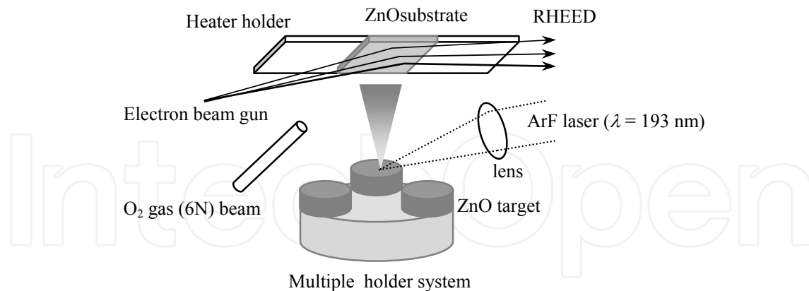
Fig. 4. A schematic figure of the laser-MBE apparatus.
