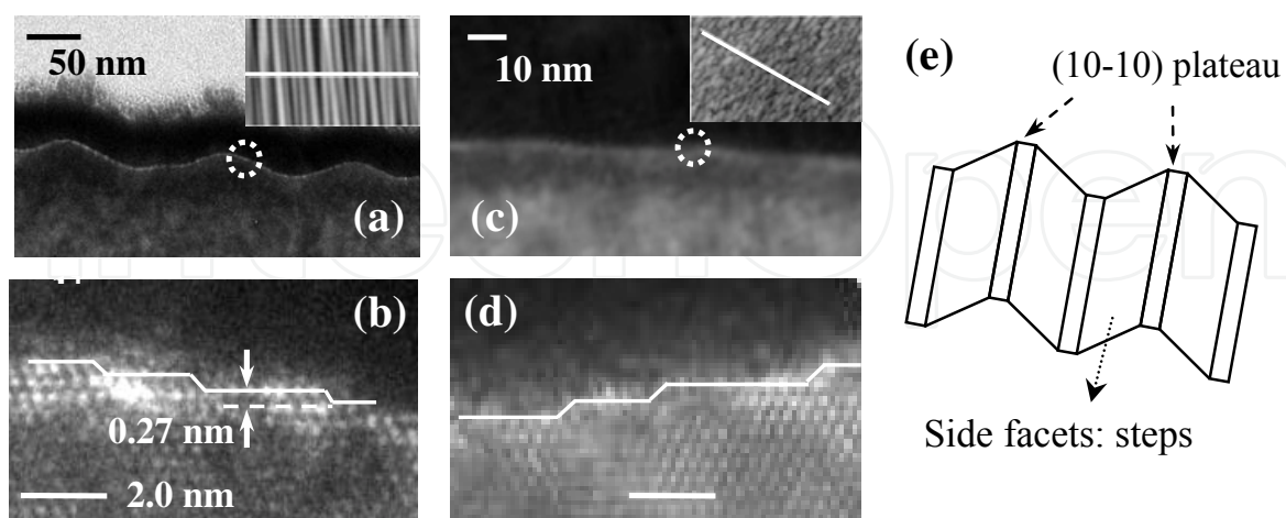
Fig. 7. (a) Low-and (b) high-resolution X-TEM images of the ZnO layer with a thickness of 240 nm. (c) Low-and (d) high-resolution X-TEM images of a 20 nm-thick ZnO layer. Insets (a) and (c) represent AFM images of the ZnO layers used for X-TEM observations. (e) Schematic representation of surface nanowires identified from X-TEM images.
