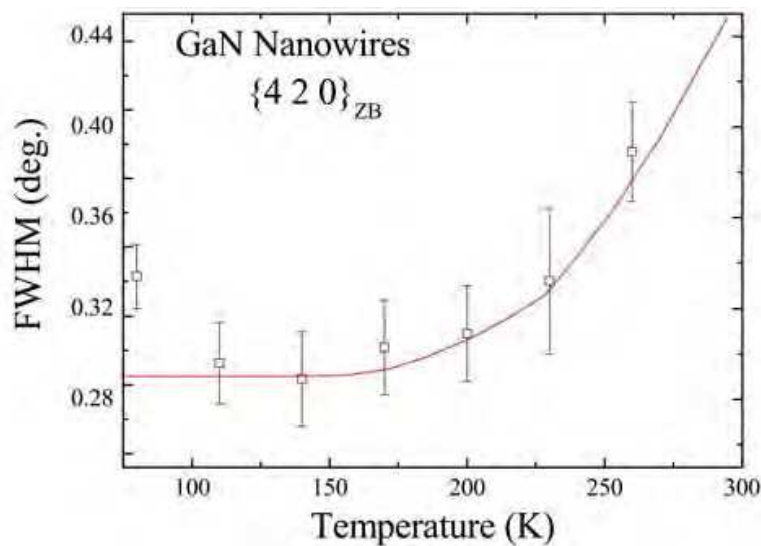
Fig. 12. Temperature dependence of the FWHM of the \{420\}_{ZB} reflection, where the solid curves is guide to the eye only. The temperature dependency of the FWHM of the selected peak of \{4 2 0\}_{ZB} indicates the structure of the ordering parameter with temperature.
