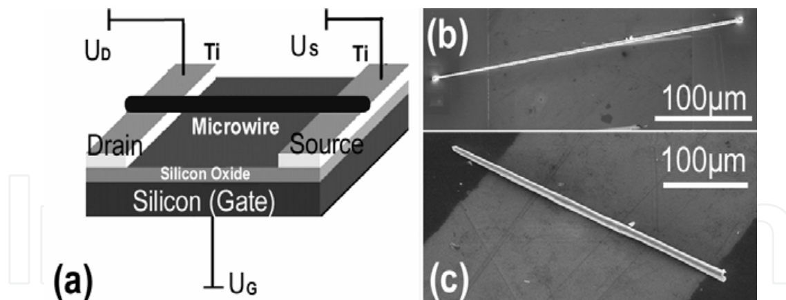
Fig. 9. (a) Schematic illustration of the back-gate FET configured with a microwire as conductive channel. (b) SEM image of an undoped ZnO microwire fixed on titanium electrodes with IBID. (c) SEM image of phosphorus doped ZnO microwire directly connecting with two titanium contacts.
