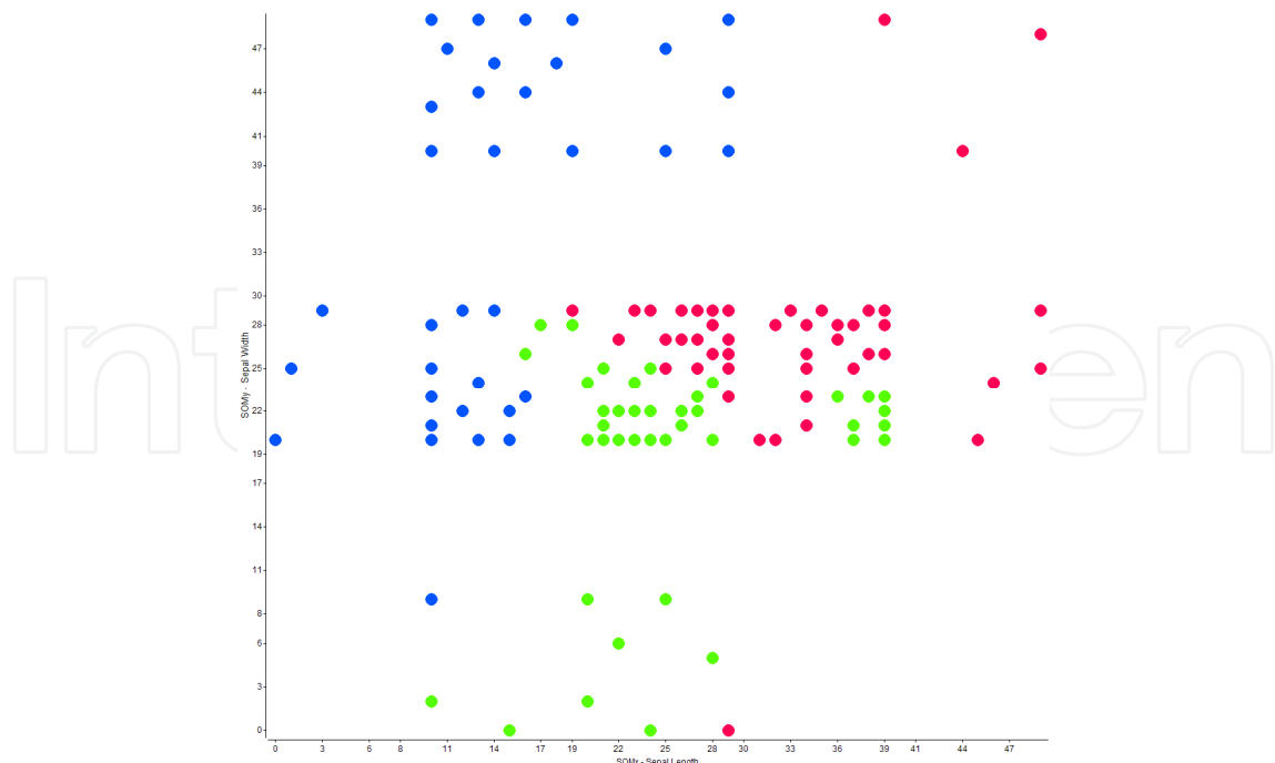
Fig. 9. SOM - Scatter plot visualization of the modified Iris flower data set with 5x5 primary and 10x10 secondary output grid
