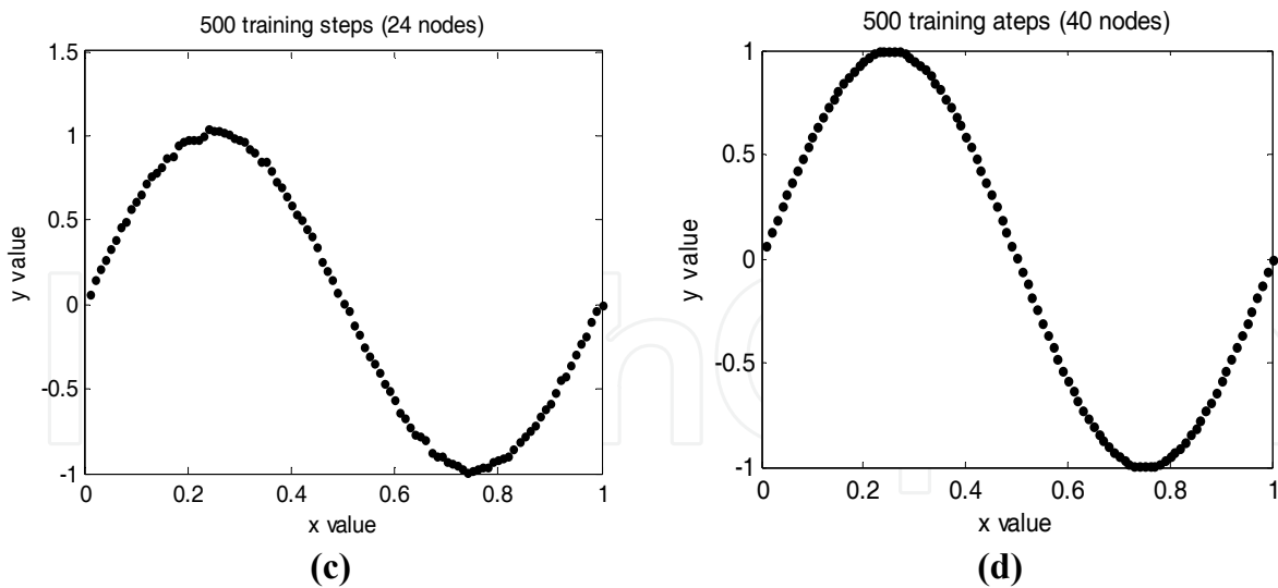
Fig. 3. The results of the sine function
