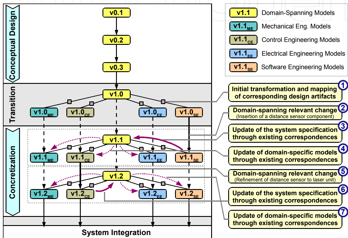
Fig. 20. Propagation of relevant changes between the domain-specific models and the domain-spanning system specification [GSD+09]
