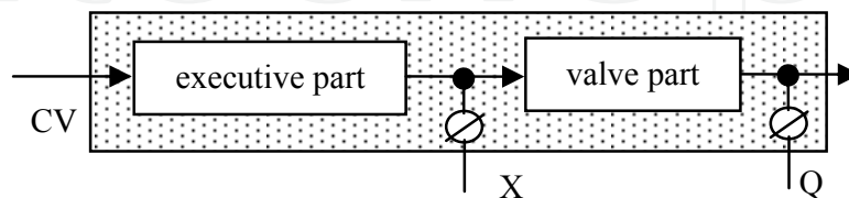
Fig. 2. Generalized model of actuator with digital positioner
