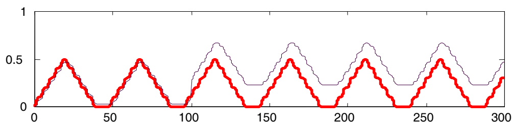
(a) signals of valve travel setting(bold line) and valve travel
