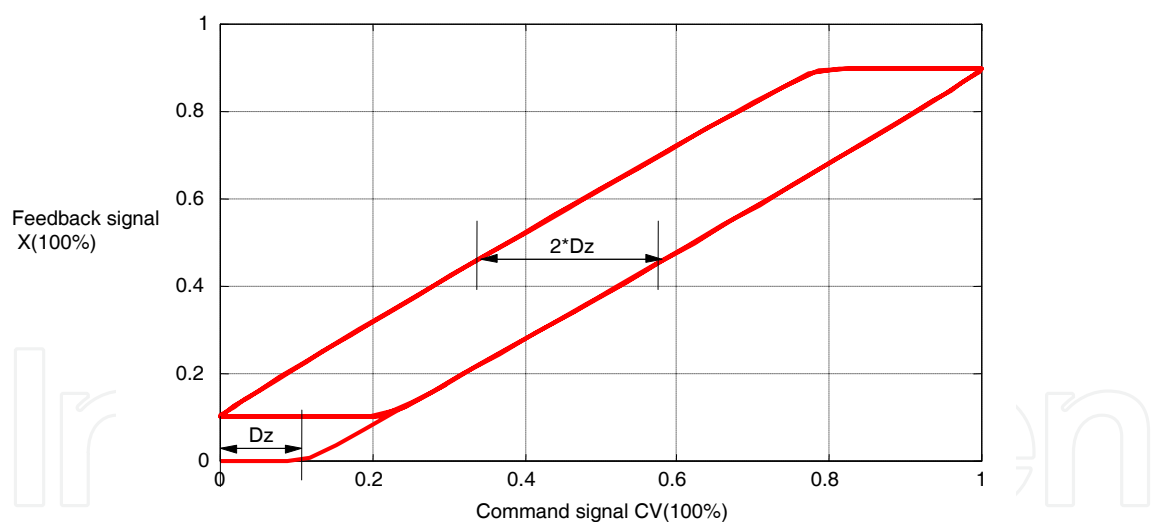
Fig. 15. X-Y graph with dead zone is D_z
