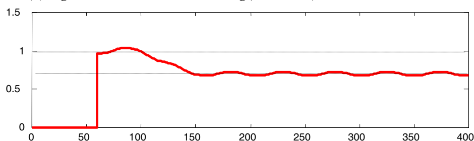
(b) estimated gain factor value of the actuator
