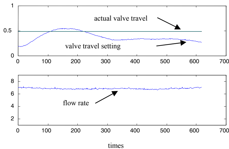
Fig. 18. Signals when the stuck fault occurs
