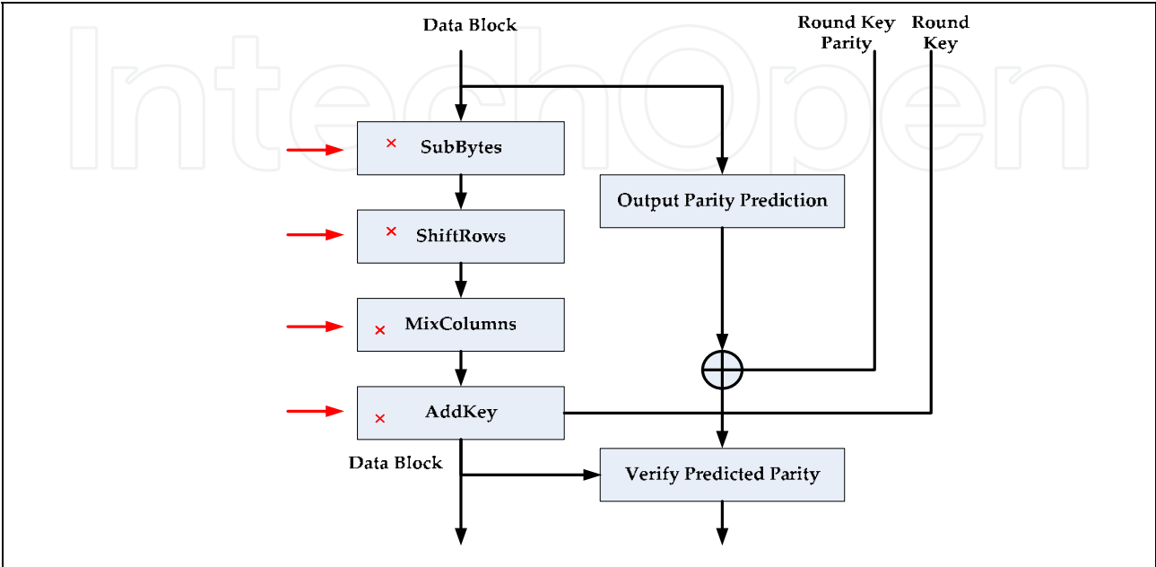
Fig. 9. Errors injection model
