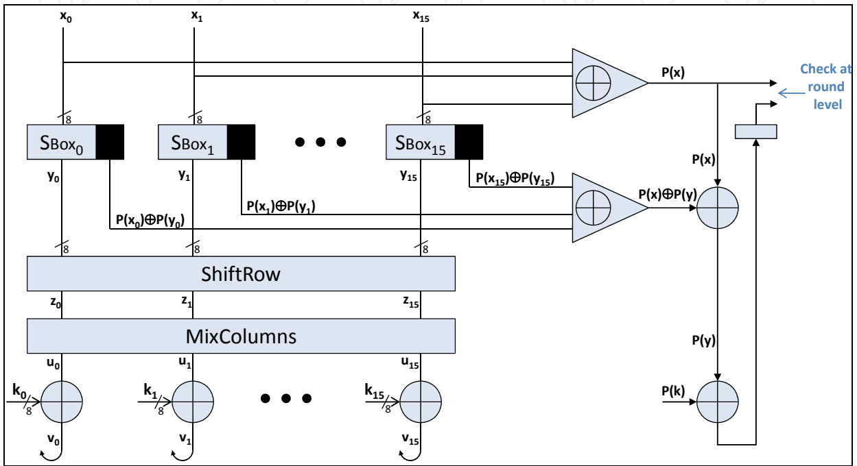
Fig. 5. (Wu et al., 2004) concurrent checking scheme
