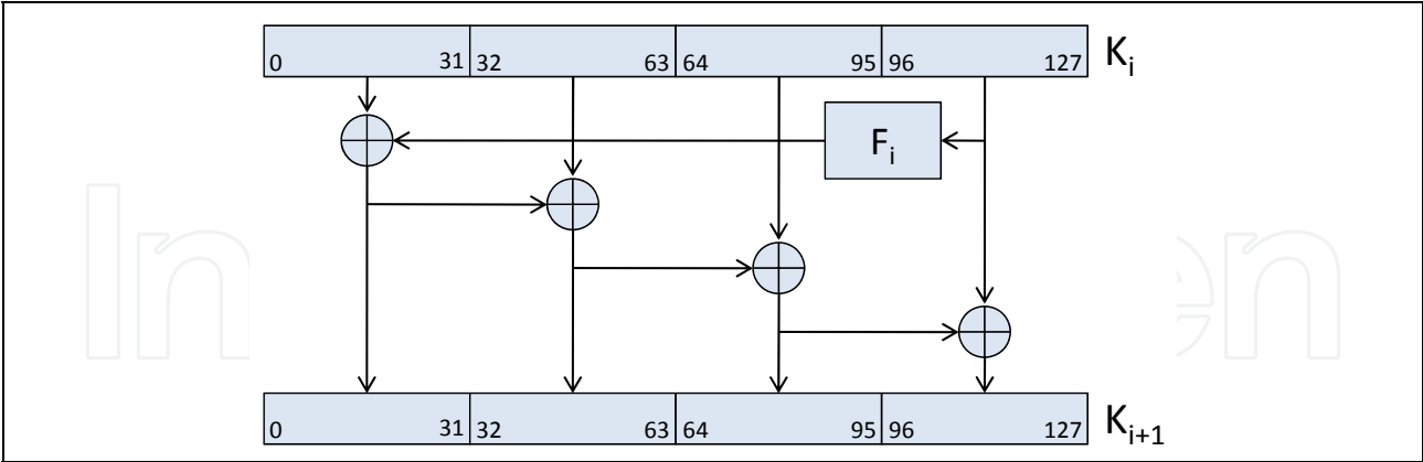
Fig. 4. AES Key Expansion Scheme
