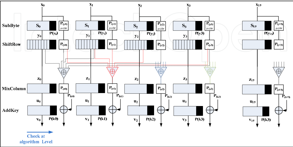
Fig. 6. AES round with (Bertoni et al., 2003) model
