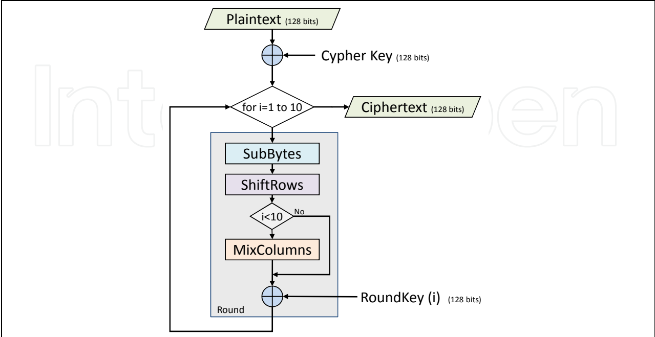
Fig. 2. AES Algorithm
