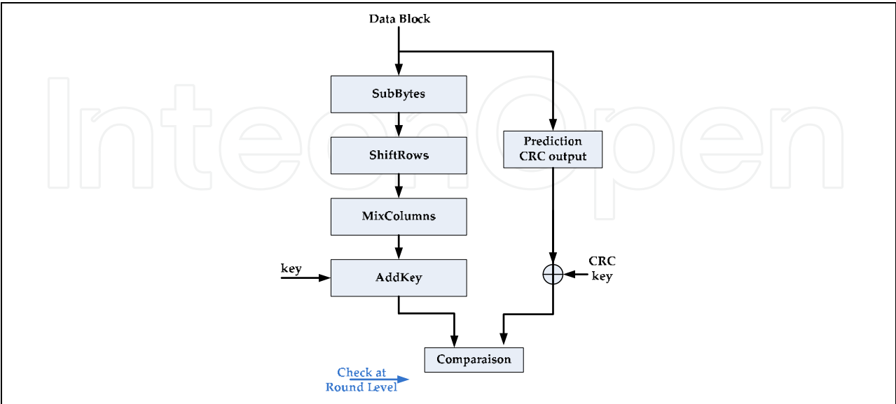
Fig. 7. AES round with (Yen and Wu, 2006) model
