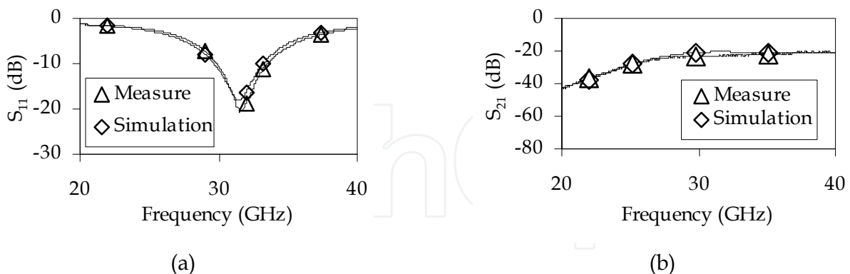
Fig. 15. Comparison between measure and simulation of S_{11} (a) and S_{21} (b) for a silicon bulk substrate of thickness 725\ \mu\text{m} and resistivity of 20\ \text{Ohm.cm} .
