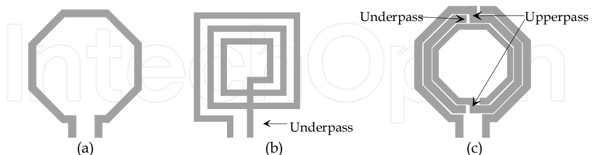
Fig. 6. (a) octagonal one turn inductor, (b) square inductor with one underpass, (c) symmetric octagonal inductor with several underpass and upperpass.
