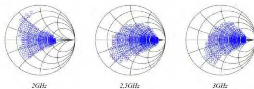
Fig. 26. Smith chart of simulated results of a CMOS AMS 0.35 \mu m device for 3 frequencies
