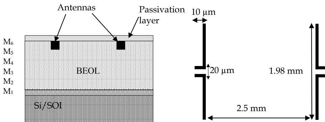
Fig. 14. Schematic view of antennas
