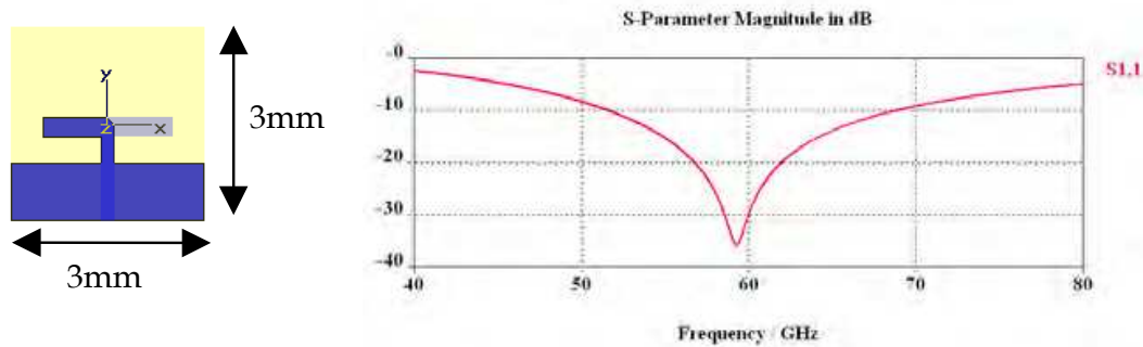
Fig. 22. Dipole antenna millimeter wave and his S_{11}
