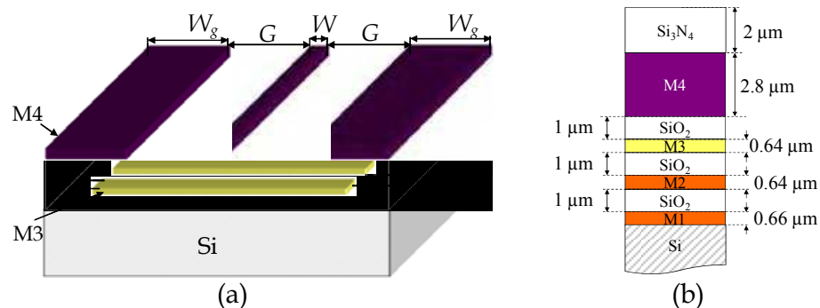
Fig. 9. (a) 3D geometric view of the slow-wave coplanar transmission line with floating metal strips. (b) Four copper metal layers 0.35- \mu\text{m} CMOS technology schematic description.
