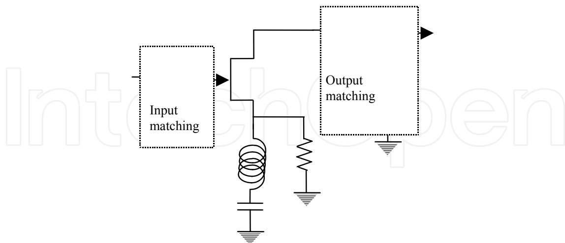
Fig. 23. Typical stand-alone MMIC amplifier with matching networks
