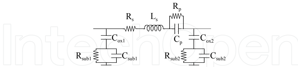
Fig. 4. The more commonly used electric model of capacitor
