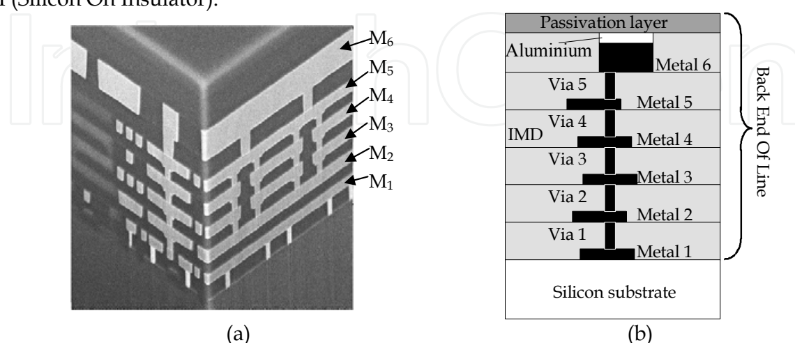
Fig. 1. BEOL with 6 interconnect levels: (a) 3D view, (b) schematic view (IMD=Inter-Metallization Dielectric)
