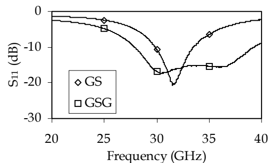
Fig. 16. Influence of probe type on reflection coefficient
