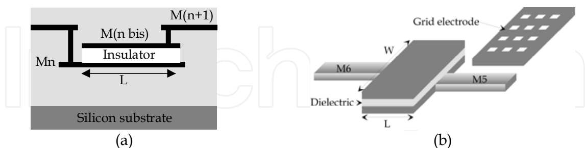
Fig. 2. Schematic view of a MIM capacitor: (a) cross-section, (b) 3D view
