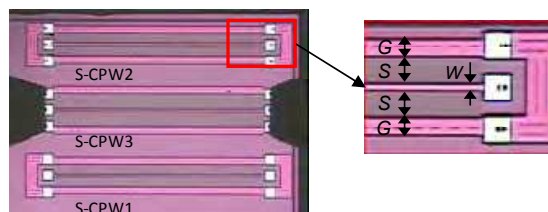
Fig. 10. Micrograph of the fabricated S-CPW transmission lines.
