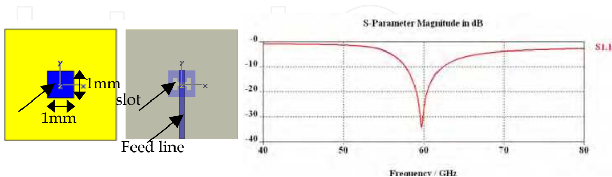
Fig. 20. Patch slot antenna millimeter wave and his S_{11}
