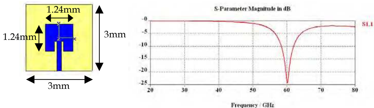
Fig. 19. Patch antenna millimeter wave and his S_{11}
