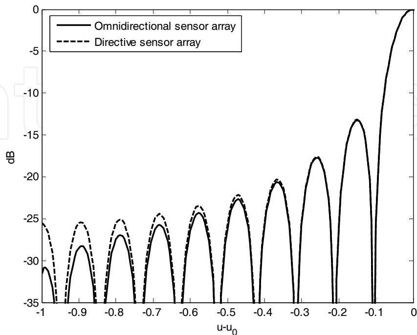
Fig. 3. Sensor directivity effect vs. |u-u_0|
