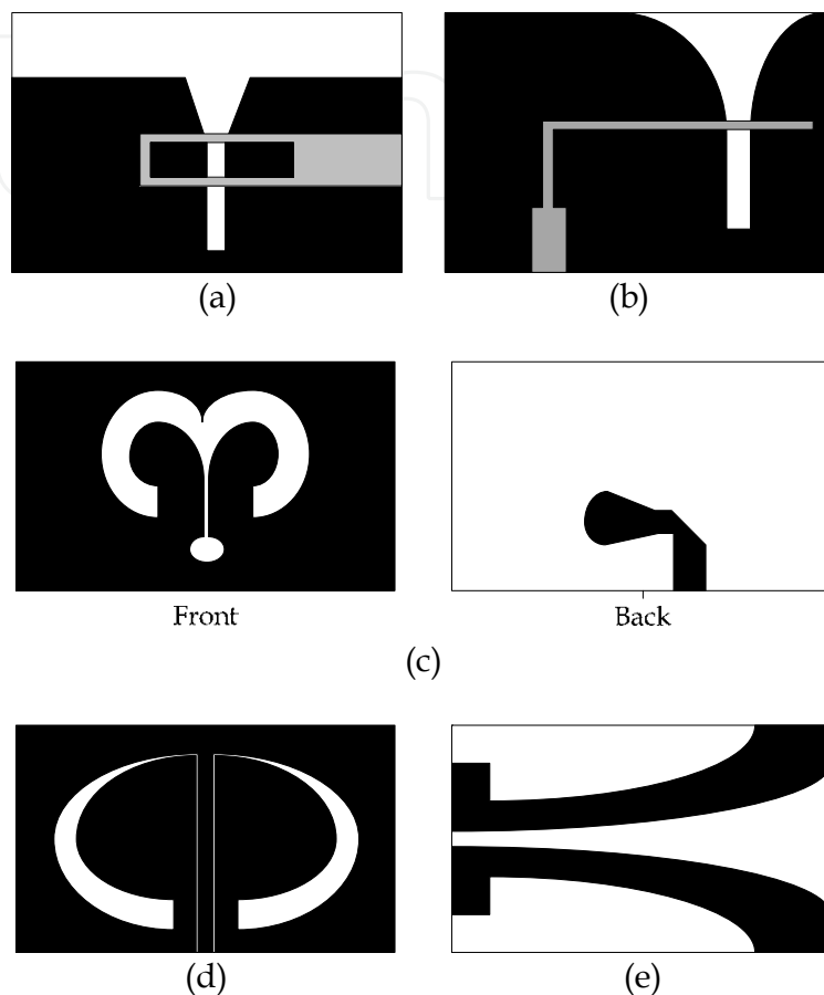
Fig. 18. The tapered slot antennas for UWB systems
