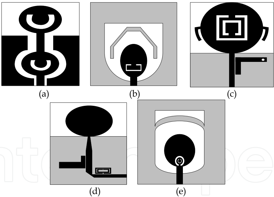
Fig. 31. Multiple band notched UWB antennas
