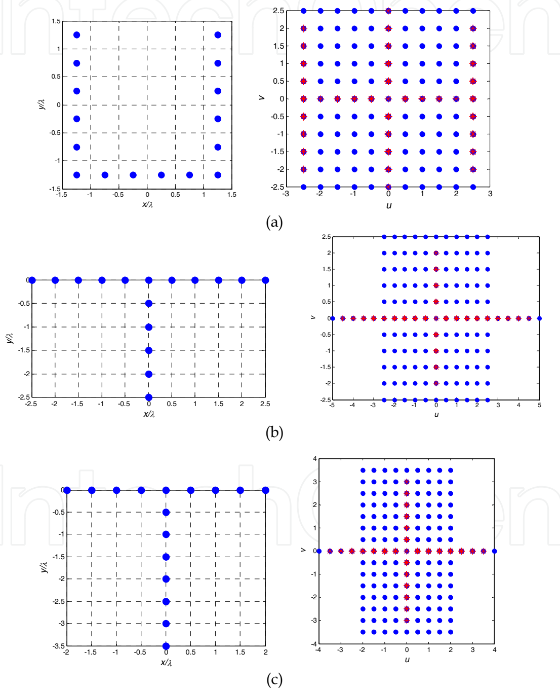
Fig. 1. Different array configurations for rectangular domain and their spatial frequency coverage. Red star points denote redundant (u, v) samples. (a) 16-element regular U-shape array; (b) 16-element regular T-shape array; (c) 16-element optimal T-shape array
