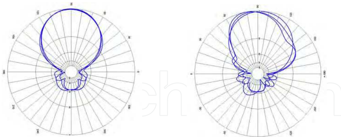
Fig. 12. (a) Horizontal Radiation Pattern
