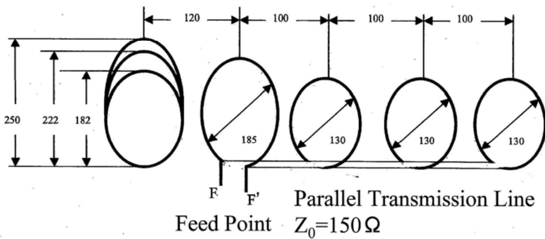
Fig. 5. Structure of RLA
