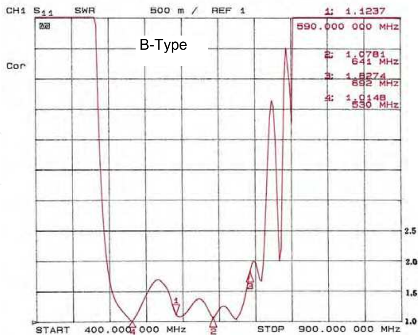
Fig. 18. Characteristics of VSWR
