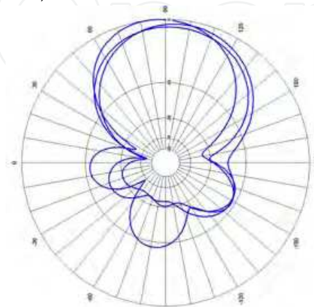
Fig.7 (b) Vertical Radiation Pattern
