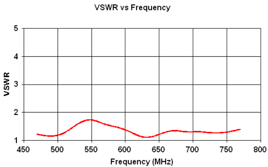
Fig. 11. VSWR characteristics of LPRLA (Theoretical Value)
