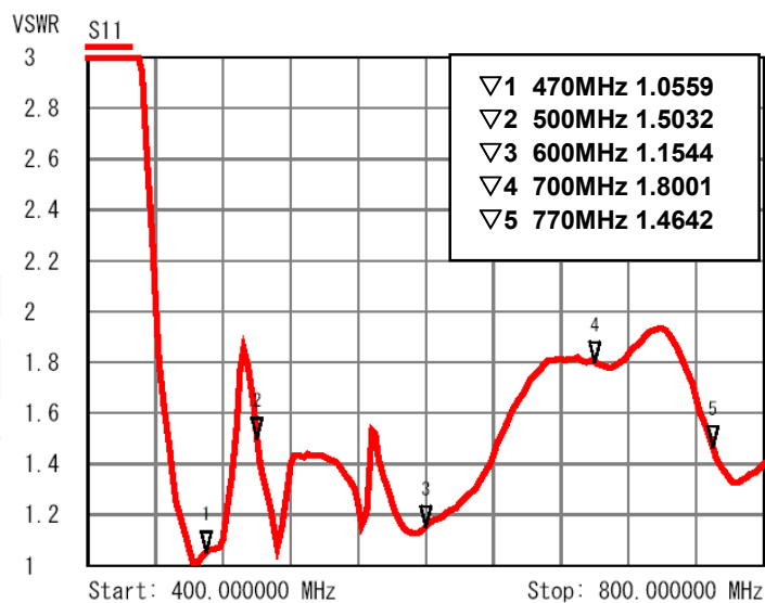
Fig. 8. VSWR characteristics of RLA (Measured Value)
