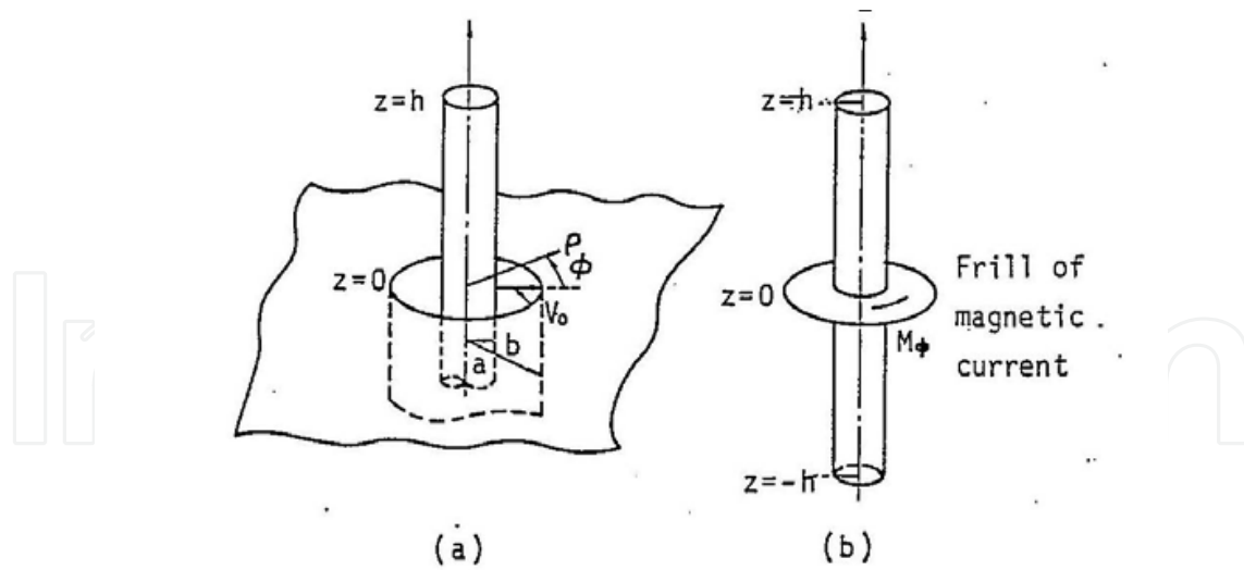
Fig. 2. Coaxial cable line feeding a monopole through a ground plane and mathematical model of the antenna
