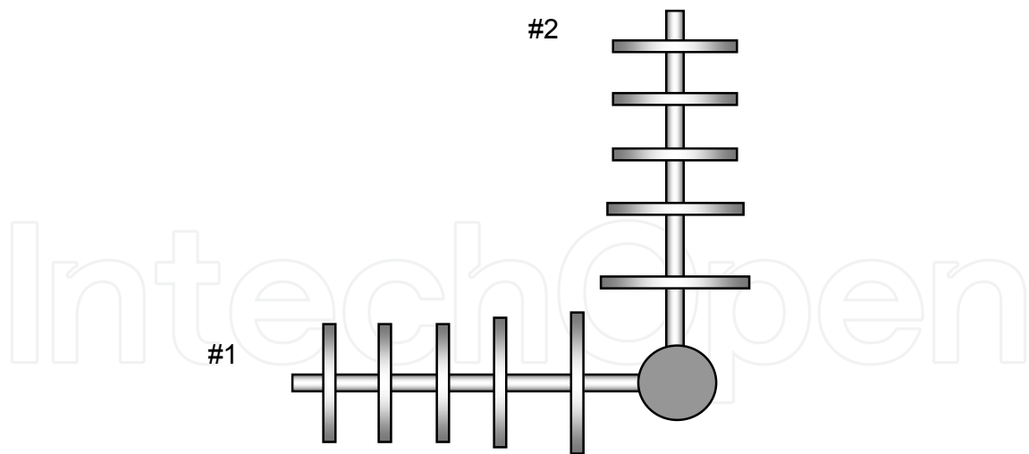
Fig. 20. Antenna arrangement
