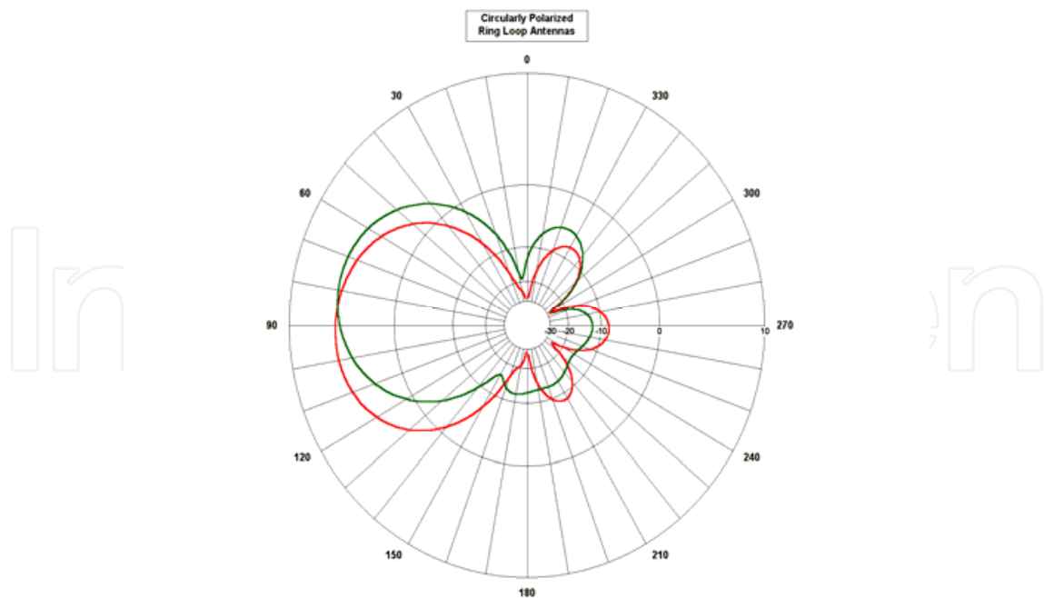
Fig. 15. Radiation Pattern of Circularly Polarized Antenna (Theoretical value) (red : horizontal, green : vertical) (Center frequency : 479MHz)
