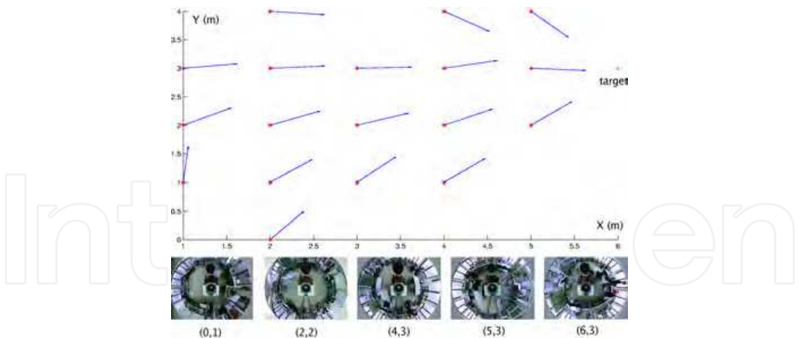
Fig. 15. Homing vectors from 1-meter-grid positions and some of the images.
