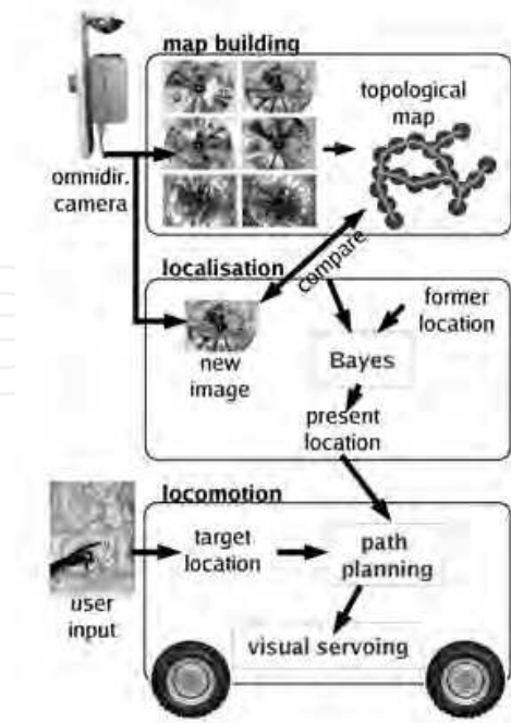
Fig. 2. Overview of the navigation method
