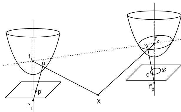
Fig. 9. Projection model for a pair of omnidirectional images.
