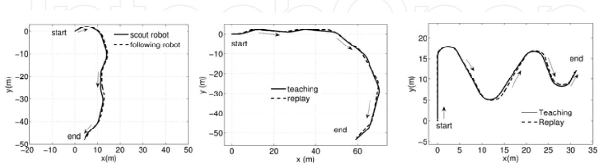
Fig. 13. LEFT: The robot followed a path taken earlier by a scout robot. MIDDLE: A path on rough terrain. RIGHT: A path with sharp turns.
