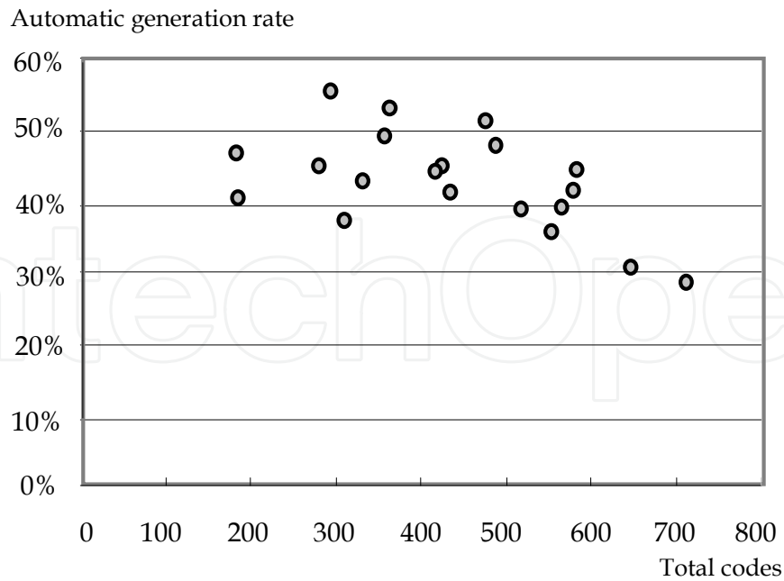
Fig. 6. Automatic code generation rate.
