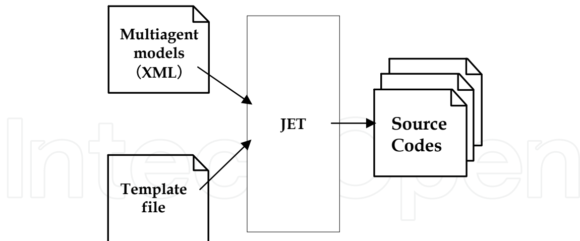
Fig. 4. Technologies for transforming models into codes.
