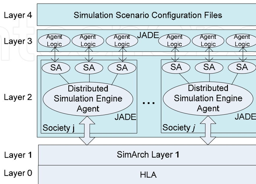
Fig. 1. The TDS architecture
