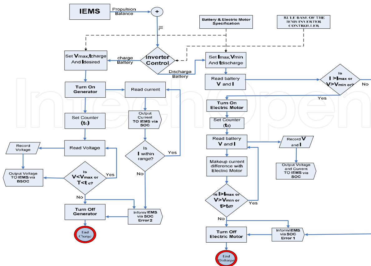
Fig. 14. Overview of the inverter algorithm.
