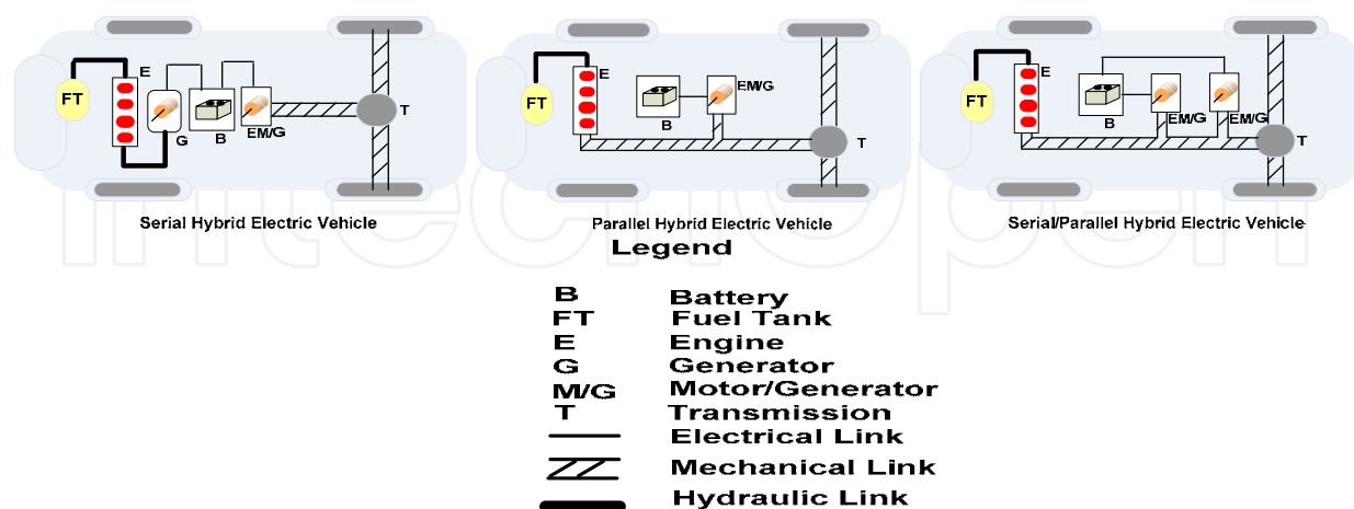
Fig. 1. Three HEVs structures.
