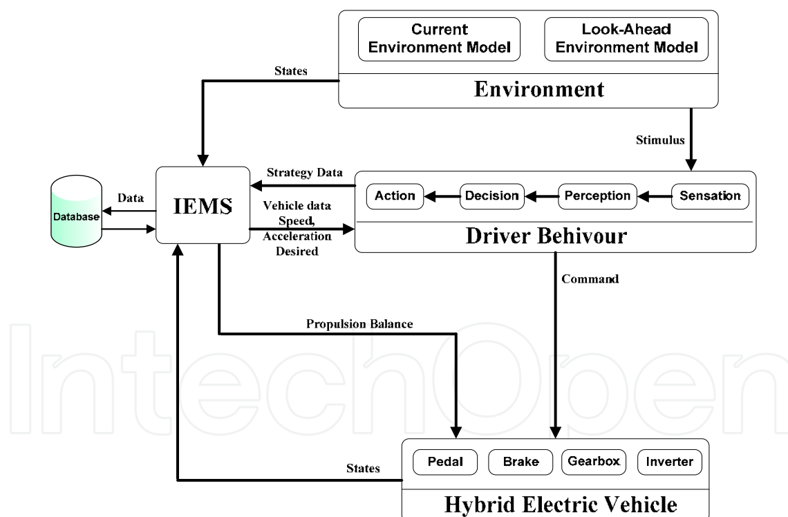
Fig. 2. Overview of the energy management model for HEVs.
