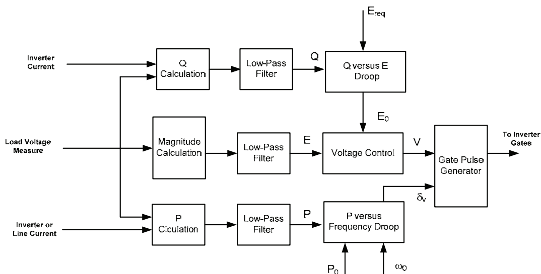
Fig. 10. Inverter control scheme proposed in (Lasseter 2002; Robert Lasseter and Piagi 2006; Lasseter 2007; Piagi and Lasseter June 2006).
