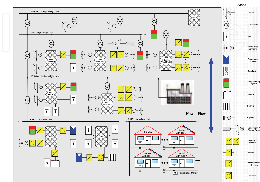
Fig. 1. Principal supply strategy of distributed Generation.
