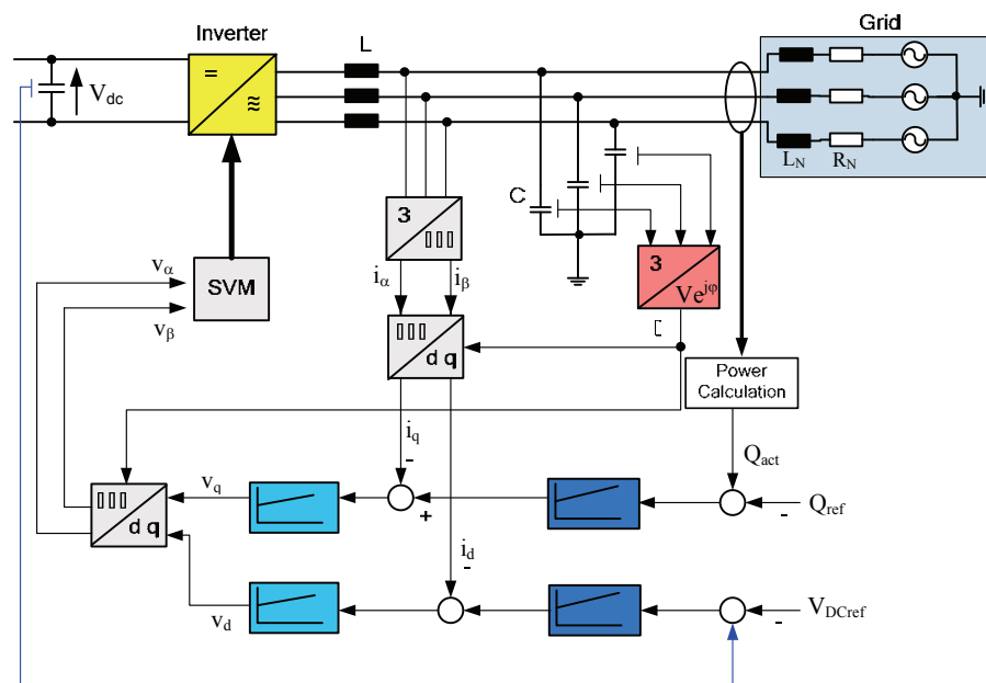
Fig. 24. Q-controlled inverter in grid parallel mode.
