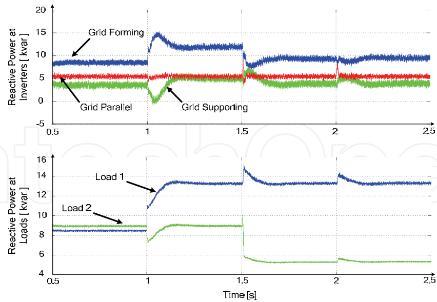
Fig. 36. The reactive power.
