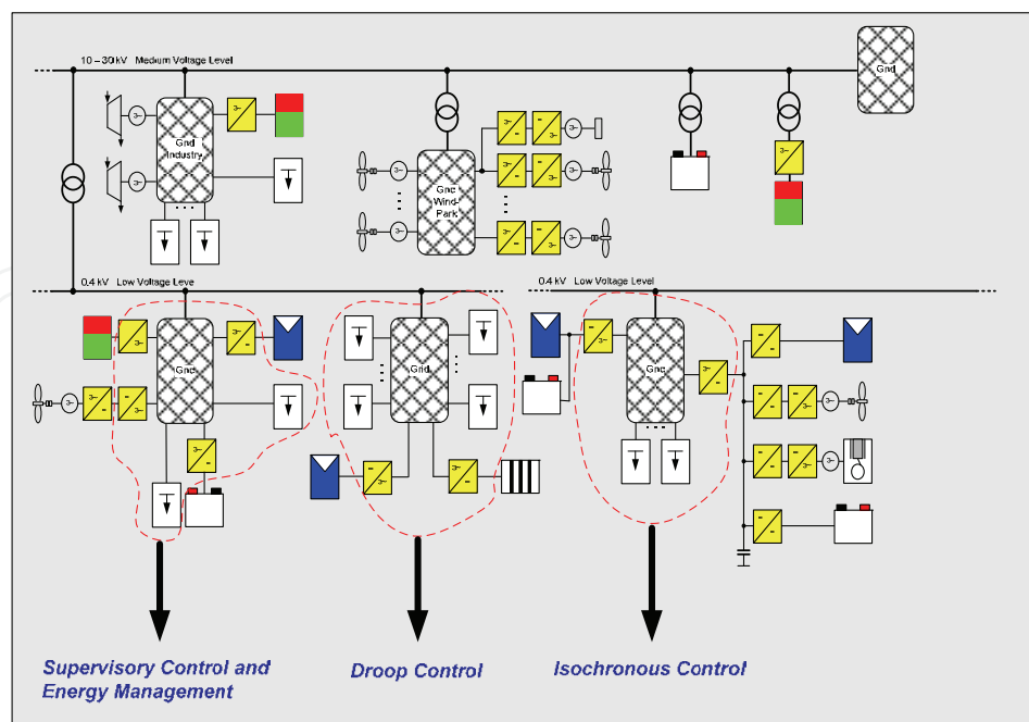
Fig. 28. The control philosophy (example).
