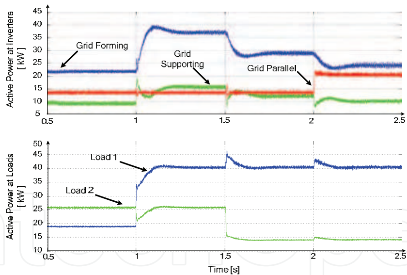
Fig. 35. The active power.
