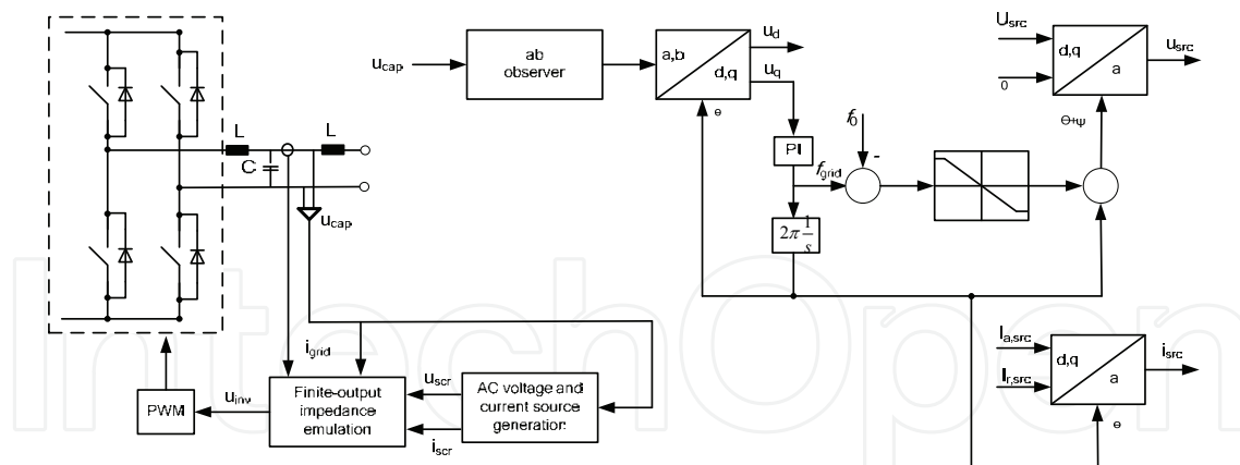
Fig. 13. Overall scheme for the proposed droop control method (Brabandere, Bolsens et al. 2004; K. De Brabandere, A. Woyte et al. 2004; De Brabandere, Vanthournout et al. 2007; Brabandere October, 2006).
