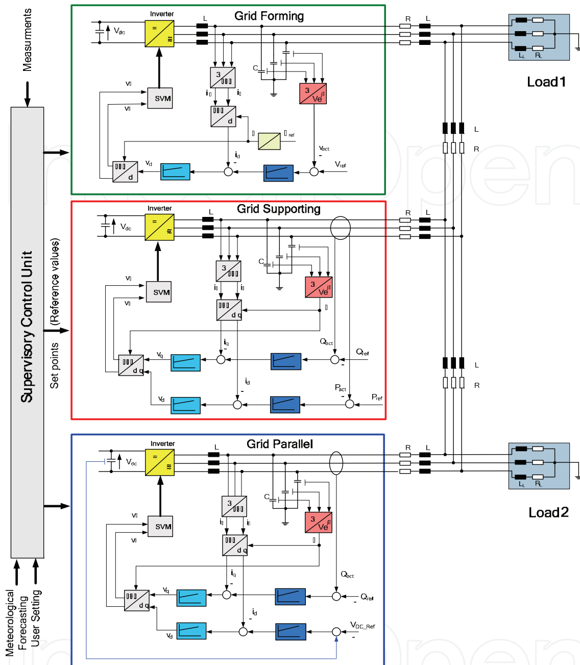
Fig. 32. Supervisory control and energy management scenario.
