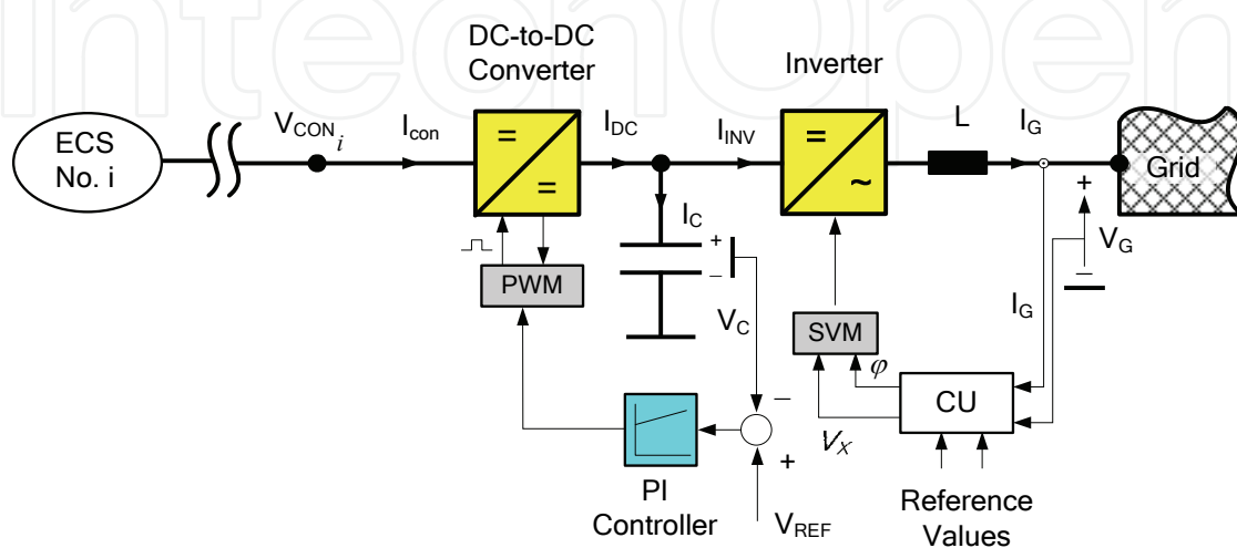
Fig. 17. General control of a system operating in a grid-driven feeding mode (Forming, Supporting).
