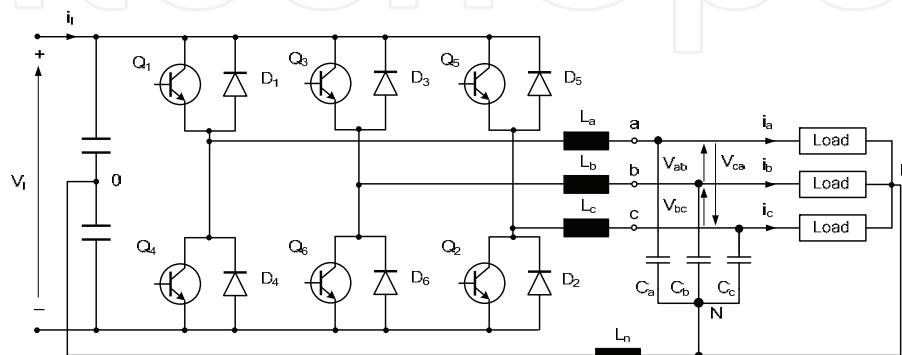
Fig. 20. Three-leg inverter with a neutral point.
