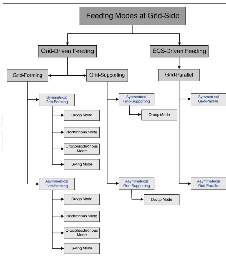
Fig. 29. Feeding modes at the grid side.
