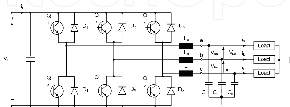
Fig. 19. Three leg inverter (balanced output).
