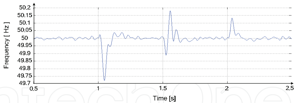
Fig. 34. The system frequency.
