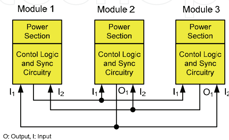
Fig. 3. Proposed Master/Slave configuration in (Petruzzello 1990)
