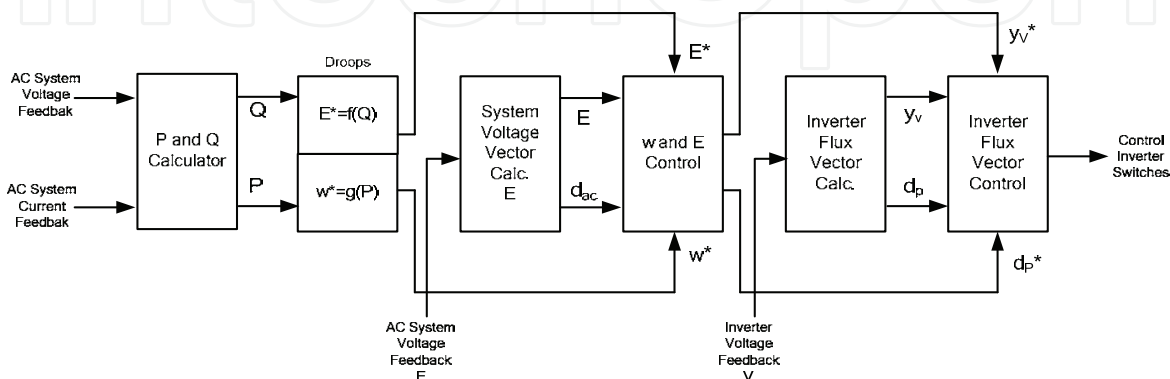
Fig. 8. Inverter control scheme (M. C. Chandorkar 1993).
