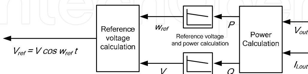
Fig. 7. Reference voltage and power calculation (C.-C. Hua).
