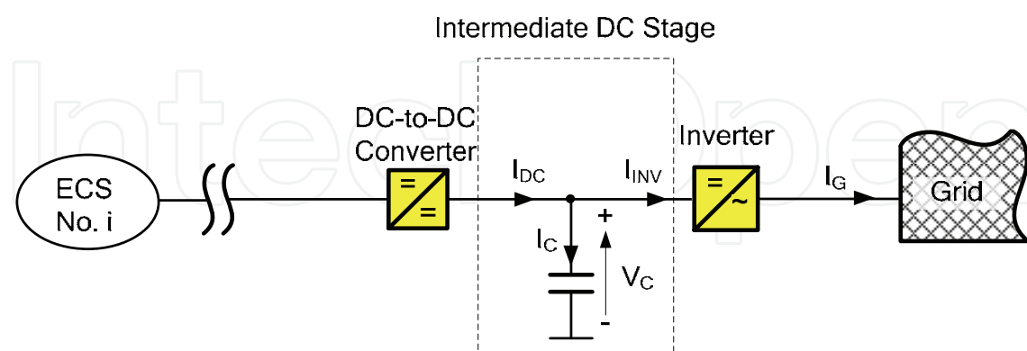
Fig. 15. System overview of the intermediate DC stage.
